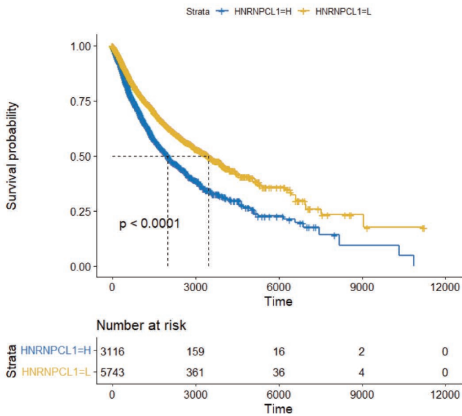
Supplementary Figure 5. Survival analysis of high expression group and low expression group of three differential SGs.
