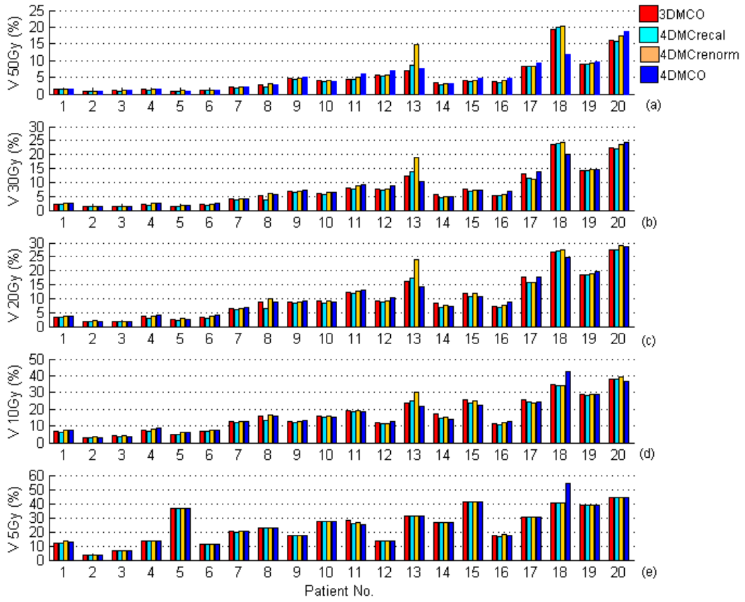
Fig. S1 Bar plot showing the percent normal lung volume receiving (a) 50 Gy, (b) 30 Gy, (c) 20 Gy, (d) 10 Gy, and (e) 5 Gy in the 3DMCO, 4DMC recal , 4DMC renorm , and 4DMCO plans in 20 patients ordered in increasing GTV size.
