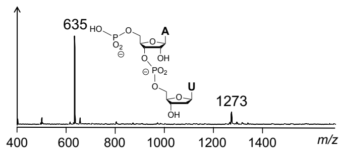
Figure S43. MALDI-TOF mass spectrum of chimeric dinucleotide 5'-pApdU.
