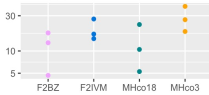
HCON_00161180:avr-15
