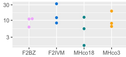
HCON_00185950:dyf-7
