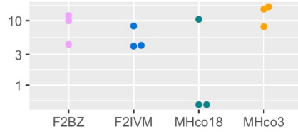
HCON_00116640:glc-6
