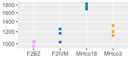
HCON_00112510:nhr-8
