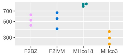
HCON_00130050:pgp-9
