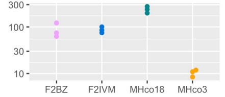
HCON_00148840:glc-3
