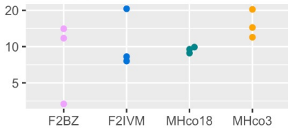
HCON_00020000:avr-14
