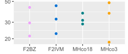
HCON_00143950:cyp-33c3
