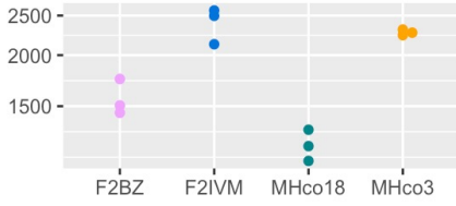
HCON_00028600:glc-5
