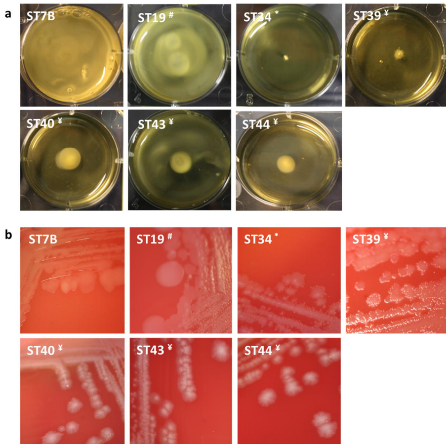
Figure S3. Motility phenotype (a) and colony morphology (b) of Clostridium botulinum isolates ST7B, ST19, ST34, ST39, ST40, ST43 and ST44. Motility assays were done in triplicate. Legend: # missense mutation in FlaA (Gln255Lys); * non-sense mutation in FlhA (Gln327*) and ¥ frame-shift insertion in FlgN (Glu3fs).
