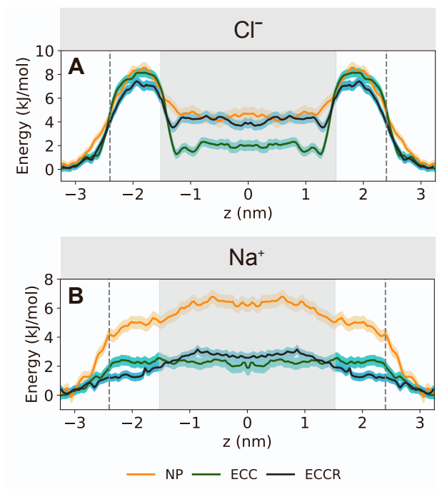
Figure S6: Single-ion PMF profiles for A \text{Cl}^- and B \text{Na}^+ permeating the model nanopore with ECC-rescaled ionic charges (green), standard non-polarizable (NP) force field (yellow) and ECCR (ECC with an additional small van der Waals radii rescaling) (dark blue). The distance between the ion and the model nanopore center of mass is denoted by z where z = 0 represents the center of the pore. The solid lines indicate the free energy profile calculated from the final 5 ns of each umbrella window. Confidence bands were calculated by taking the standard error over independent 1 ns sampling blocks over the time period sampled. The dashed vertical lines denote the extent of the nanopore.
