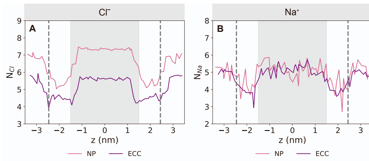
Figure S2: Variation in the first hydration shell of \text{Cl}^- (A) and \text{Na}^+ (B) as a function of z , the distance between the ion and the model nanopore center of mass. N_{\text{Cl}} and N_{\text{Na}} denote the coordination number of water-oxygen atoms in the first hydration shell of \text{Cl}^- and \text{Na}^+ respectively, with ECC-rescaled ions (purple) and a non-polarizable (NP) force field (pink). The dashed vertical lines denote the extent of the nanopore.
