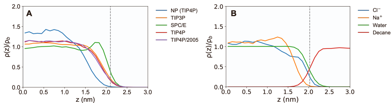
Figure S7: Symmetrized number density ( \rho(z)/\rho_b ) profiles for \text{Cl}^- (A) at an aqueous/decane interface employing various water models with ECC-rescaled charges and a non-polarizable (NP) force field using TIP4P water model. B shows the symmetrized number density profiles for \text{Cl}^- , \text{Na}^+ and water using the AMOEBA polarizable force field with the AMOEBA03 water model. The variable z is the distance from the center of the simulation box and the vertical dashed line denotes the aqueous/decane interface.
