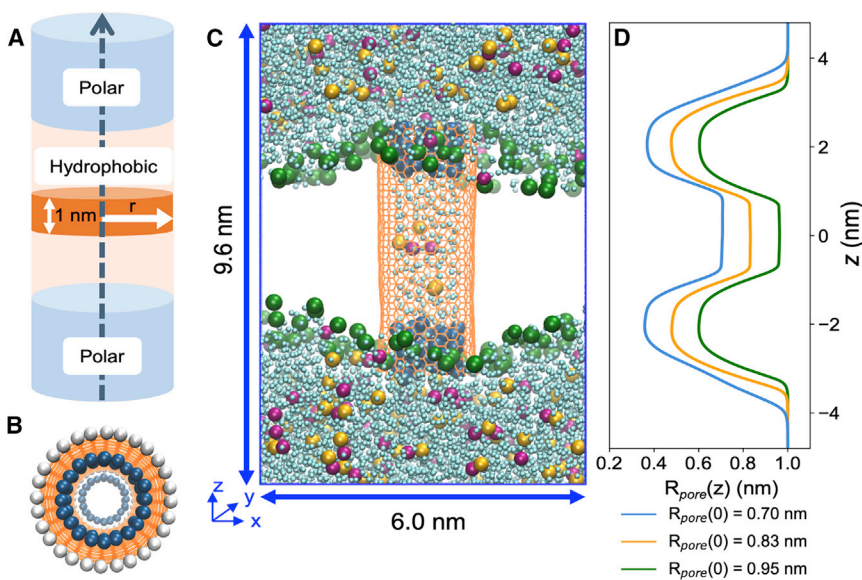
FIGURE 1 (A) Schematic of a biomimetic nanopore. The model nanopore has a radius r , such that 0 < r < R_{pore} . (B) Top-down view of the pore, showing water molecules (blue) restrained to the CNT pore walls (orange) to create the polar regions at each mouth of the pore. The nanopore ends are capped with hydrogen atoms (white). (C) Snapshot of the simulation setup. The biomimetic nanopore is embedded in a palmitoyl-2-oleoyl- sn -glycero-3-phosphocholine bilayer (lipid headgroup phosphates in green) and solvated with water (light blue), \text{Cl}^- (yellow), and \text{Na}^+ (pink). (D) Pore-radius profile showing the maximum value of R_{pore} as a function of axial position z (approximately aligned with the simulation snapshot in (C)). To see this figure in color, go online.
