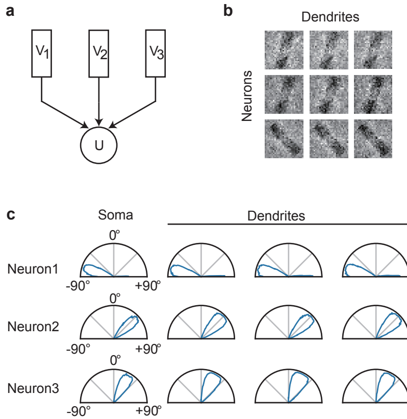
S9 Fig. Multi-dendrite neuron model without gating. (a) A schematic illustration of the neuron model with three dendritic compartments without gating. (b) Trained weight matrices are displayed for afferent inputs to three dendritic branches of three example neurons. (c) Somatic and dendritic activities of the three neurons in (b) are shown.
