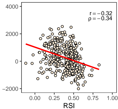
SARC
