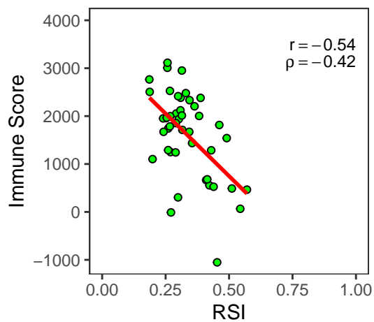
HNSC
