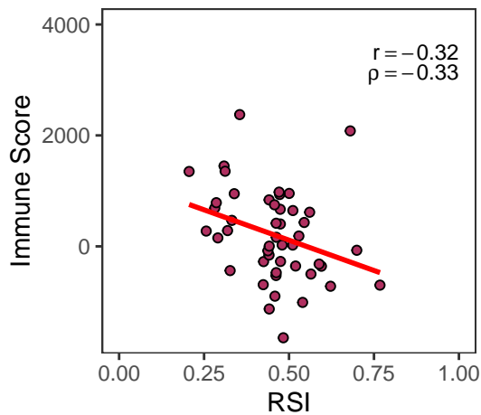
LUSC
