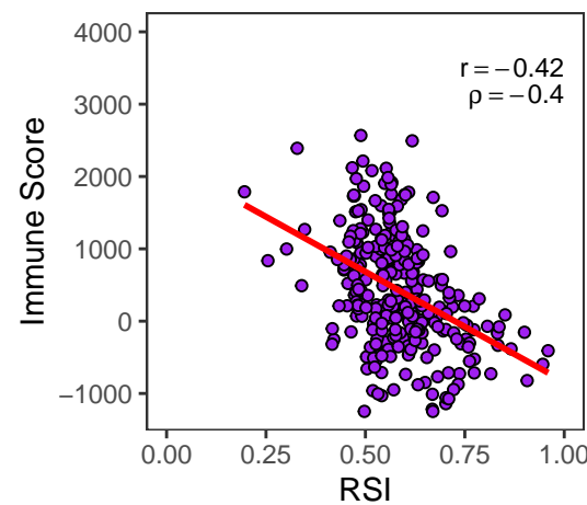
UCEC
