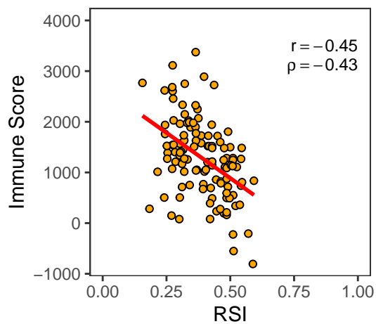
LGG
