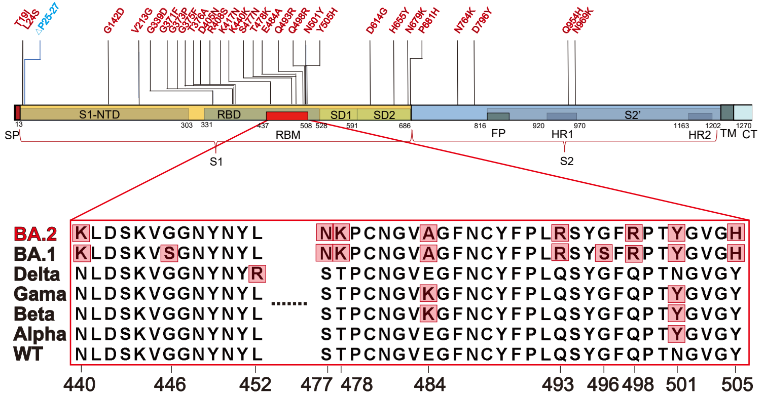
Fig. S1. Schematic of the Omicron BA.2 spike protein domain architecture.
