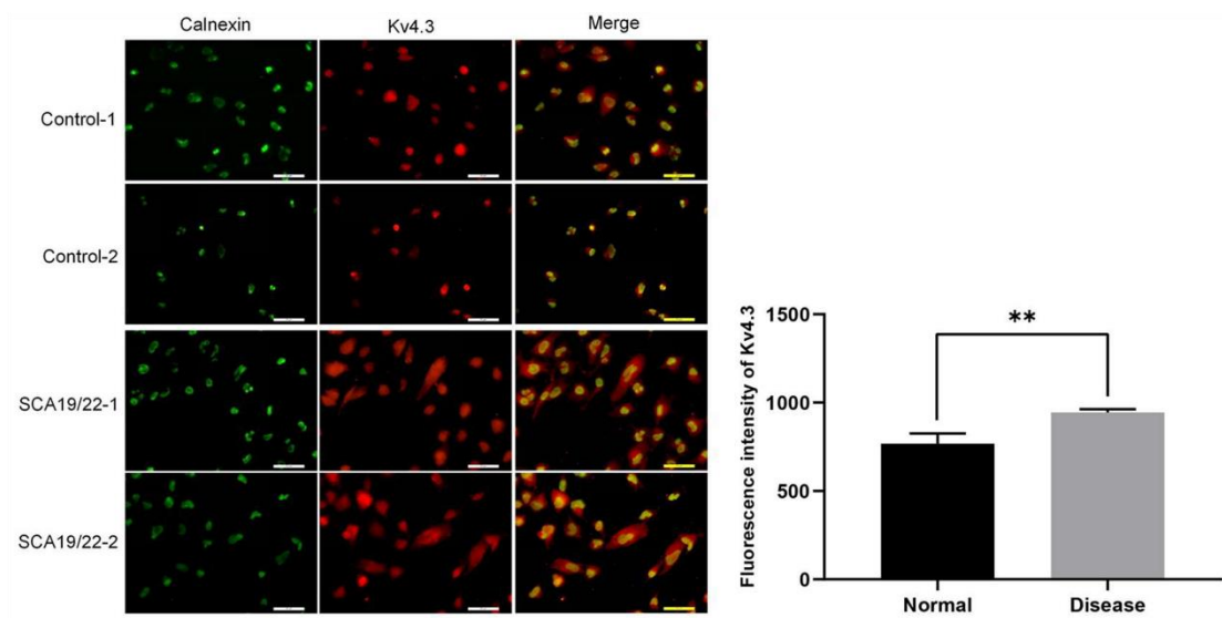
Supplement Fig. 1: Left: Colocalization with the ER marker calnexin (in green) revealed that mutant Kv4.3 proteins (in red) were retained in the ER, as was shown by the merged picture (in yellow). Scale bars 50um. Right: The results of fluorescence intensity analysis showed that more Kv4.3 was trapped in the NPCs in the disease group.
