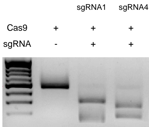
Fig. S1. In vitro cleavage assay of two different sgRNAs targeting the PPT synthase locus. A PCR fragment containing the targeted PPT synthase gene sequence was synthesized and mixed with Cas9 and each sgRNA (sgRNA1 and sgRNA4). A negative control that lacked sgRNA was included for comparison. Cleavage efficiency was assessed by agarose gel electrophoresis.
