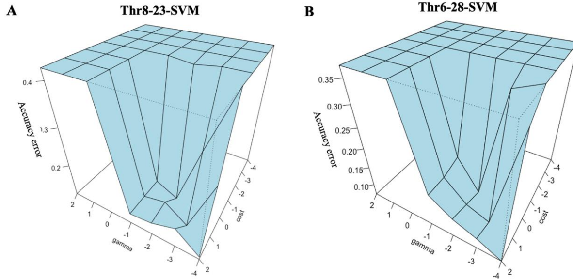
Supplementary Figure 1. Hyperparameter tuning plot of 2 SVM classifiers. Hyperparameters were tuned with gamma and cost value. Performance of the Thr8-23-SVM (A) and Thr6-28-SVM (B) measured by accuracy error were plotted. Both the gamma value and cost parameter C were tested for 0.0001,0.001,0.01,0.1,1.0,10, and 100. Both parameters were transformed by log10.
