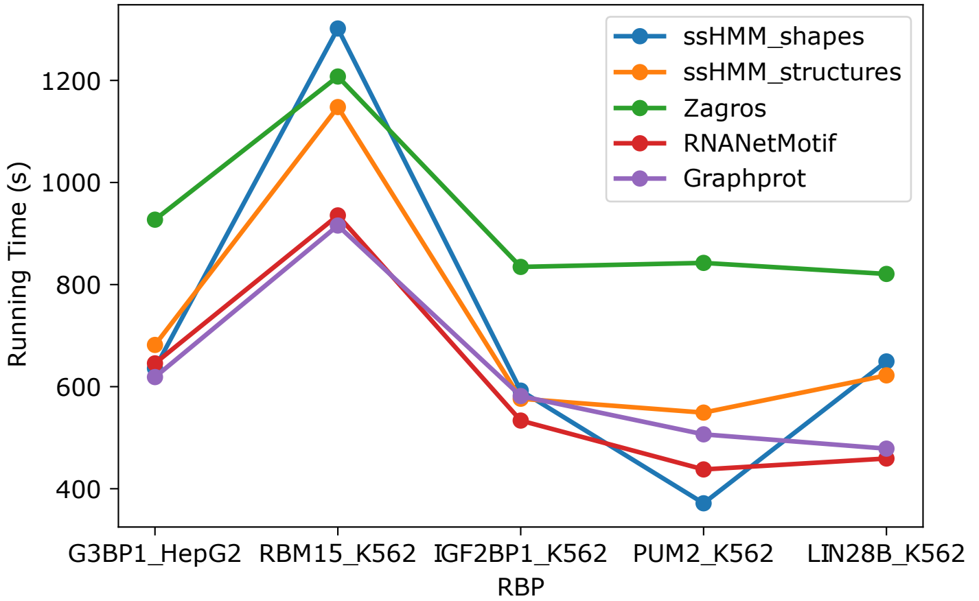
Comparison on running time of different tools
