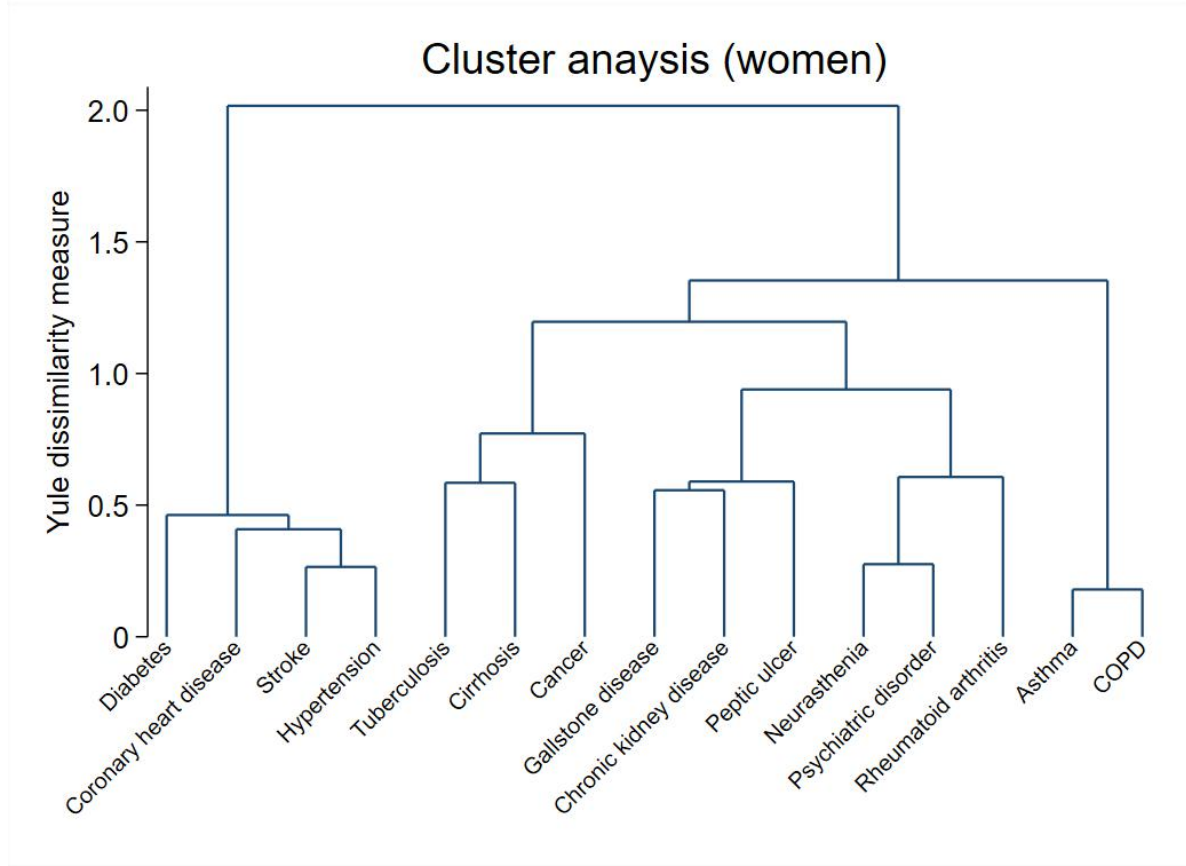
Supplementary Figure 2: Dendrograms of cluster analysis for men and women.
