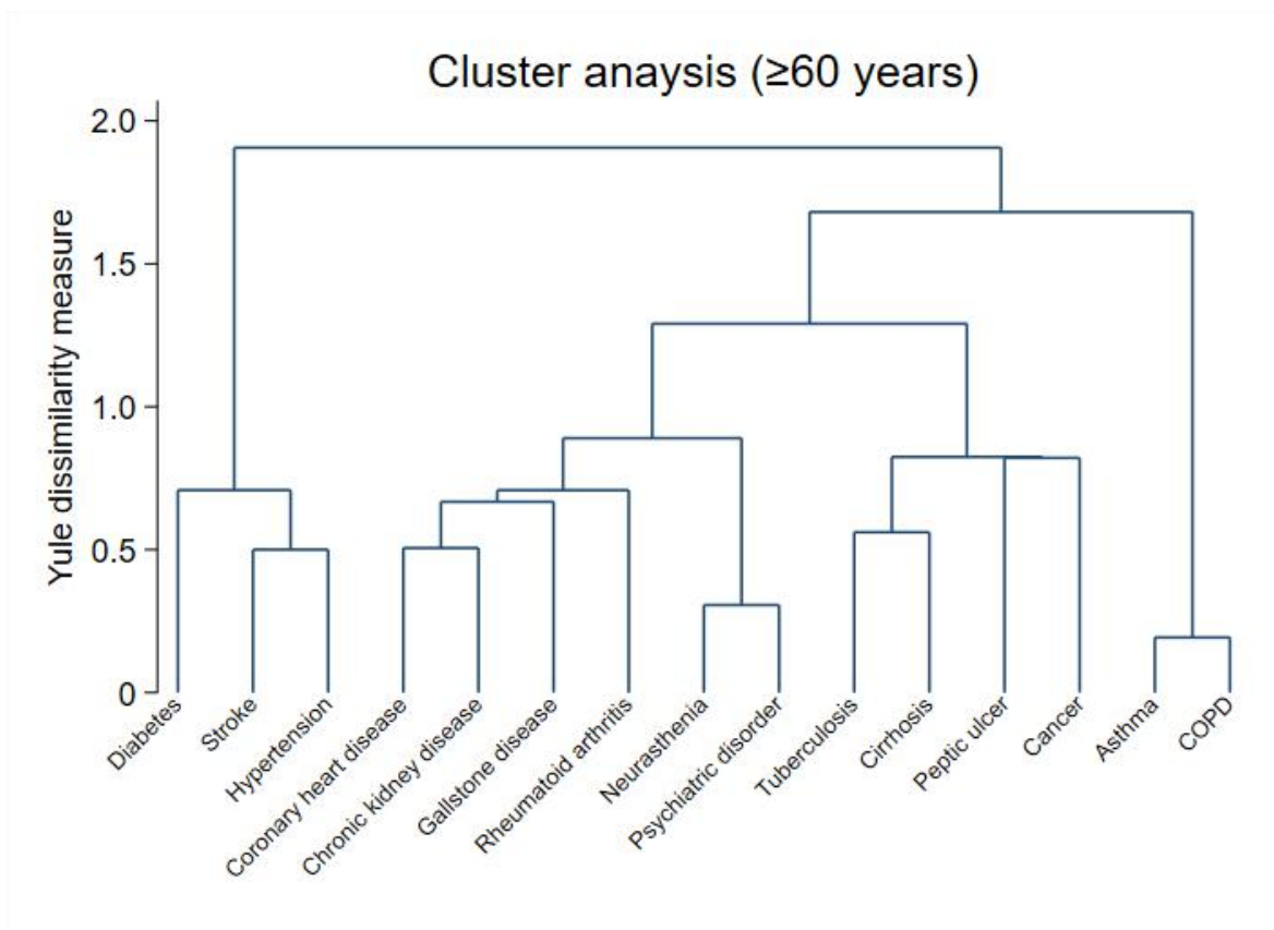
Supplementary Figure 3: Dendrograms of cluster analysis for different age groups.
