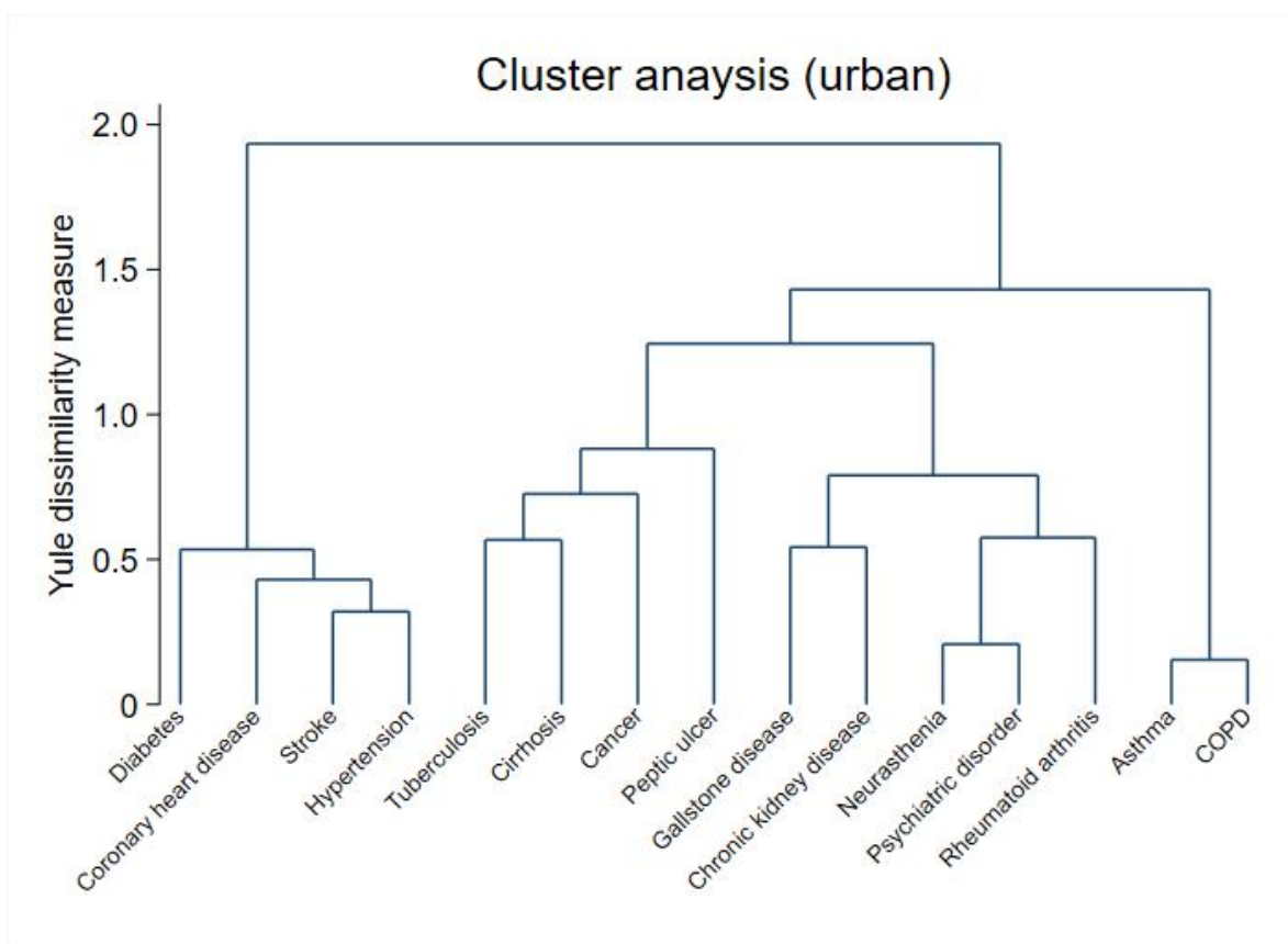
Supplementary Figure 4: Dendrograms of cluster analysis for rural and urban participants.
