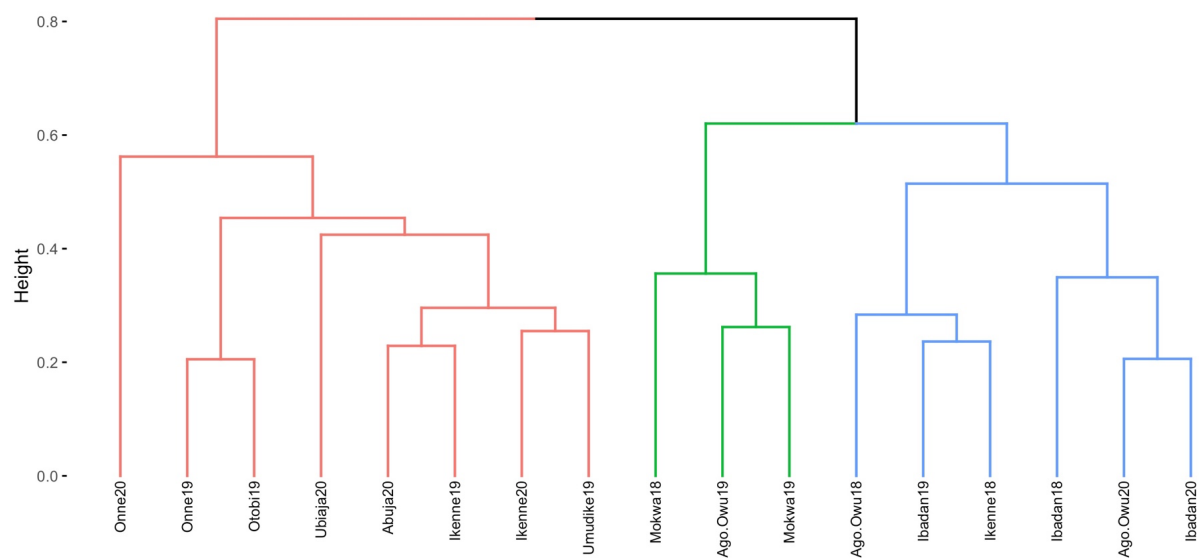
S7 Fig. A cluster dendrogram showing relatedness among the testing environments based on distance matrix derived from correlation among environments genotypic BLUPs of fresh root yield (t/ha). The clustering was based on ward.D2 linkage method.
