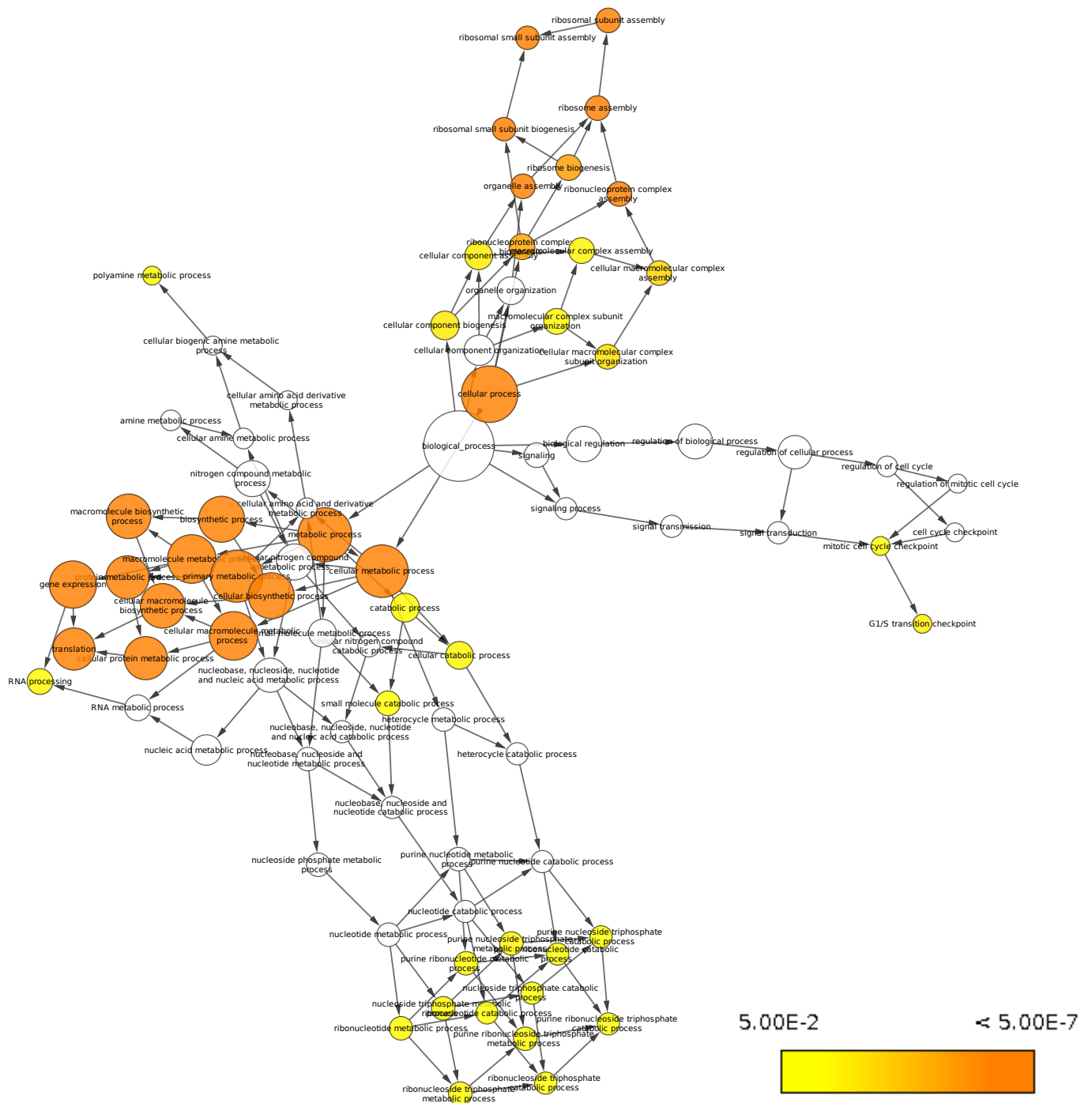
Supplementary Figure 6. Gene ontology and associated pathway network analyses: upregulated pathways in hybrids relative to murine HL1cm. Network analysis shows the upregulated GO pathways in the fusion products compared to the murine HL1cm. The size of the node denotes the number of genes included in the pathway. The yellow to orange color scale indicates significant pathways (Benjaminin-Hochberg corrected P value < 0.05), where orange color indicates higher significance.
