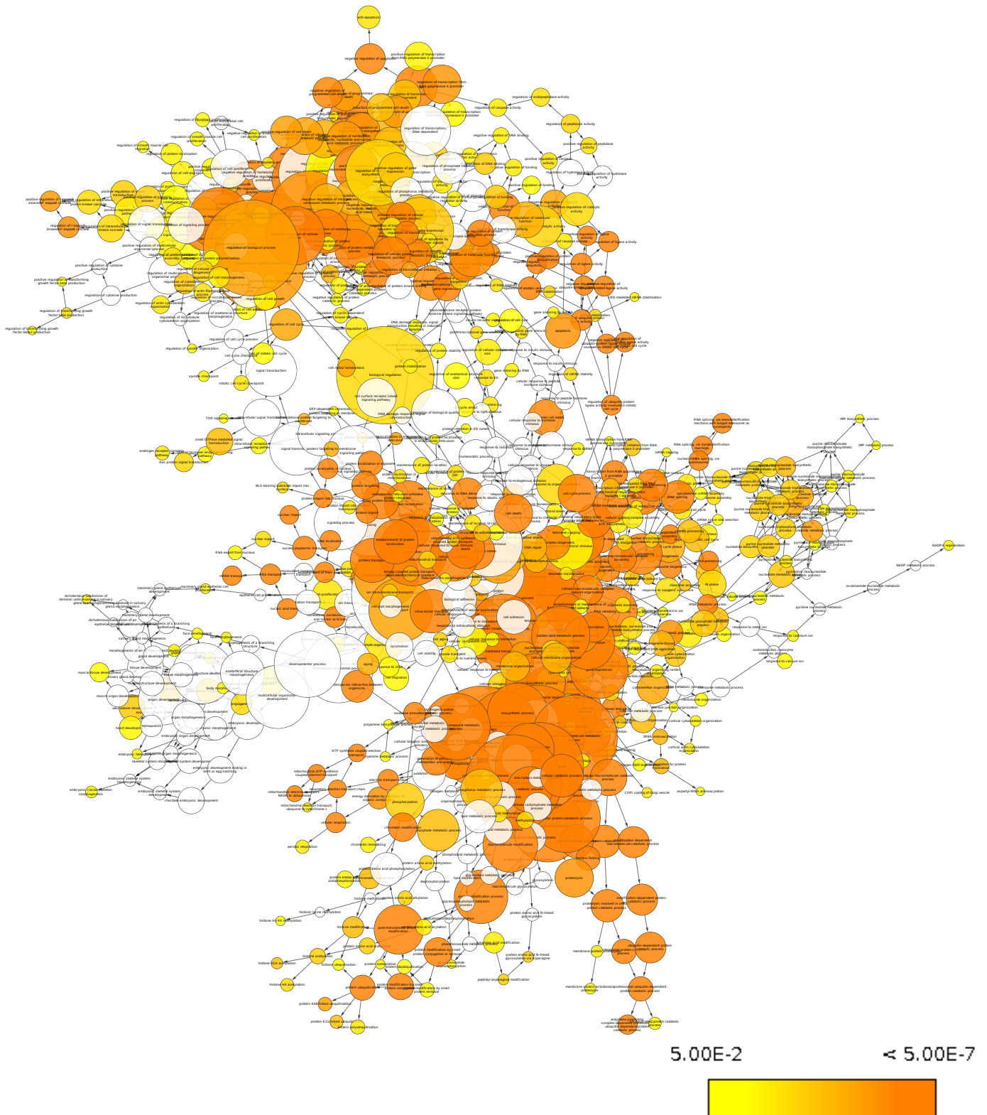
Supplementary Figure 5. Gene ontology and associated pathway network analyses: downregulated pathways in hybrids relative to hMSCs. Network analysis shows the downregulated GO pathways in the fusion products compared to the hMSCs. The size of the node denotes the number of genes included in the pathway. The yellow to orange color scale indicates significant pathways (Benjamini-Hochberg corrected P value < 0.05), where orange color indicates higher significance.
