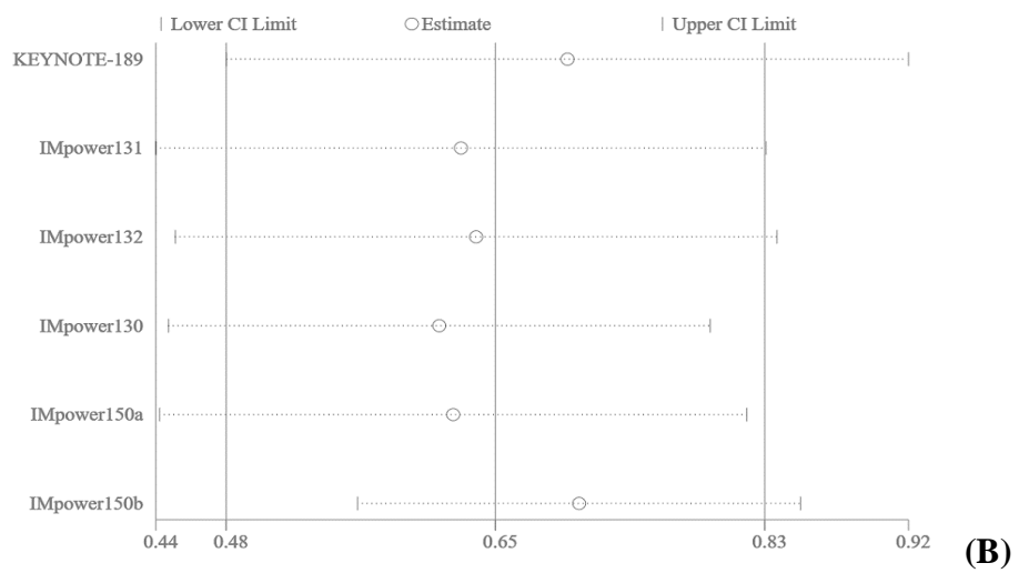
S2 Fig. Forest plot of leave-one-out approach on OS-HR (A) and PFS-HR (B). HR, hazard ratio; OS, overall survival; PFS, progress-free survival.
