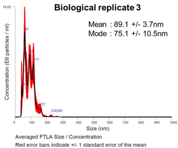
S2 Fig. Hydrodynamic size distribution profiles of isolated exosome measured by NTA.
