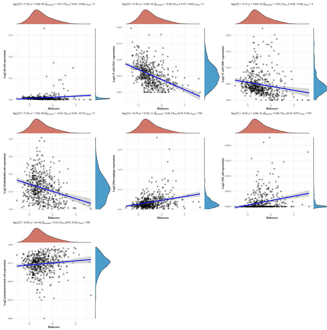
Fig.S4.1 The correlation of CRG_score with immune cells was analyzed using EPIC
