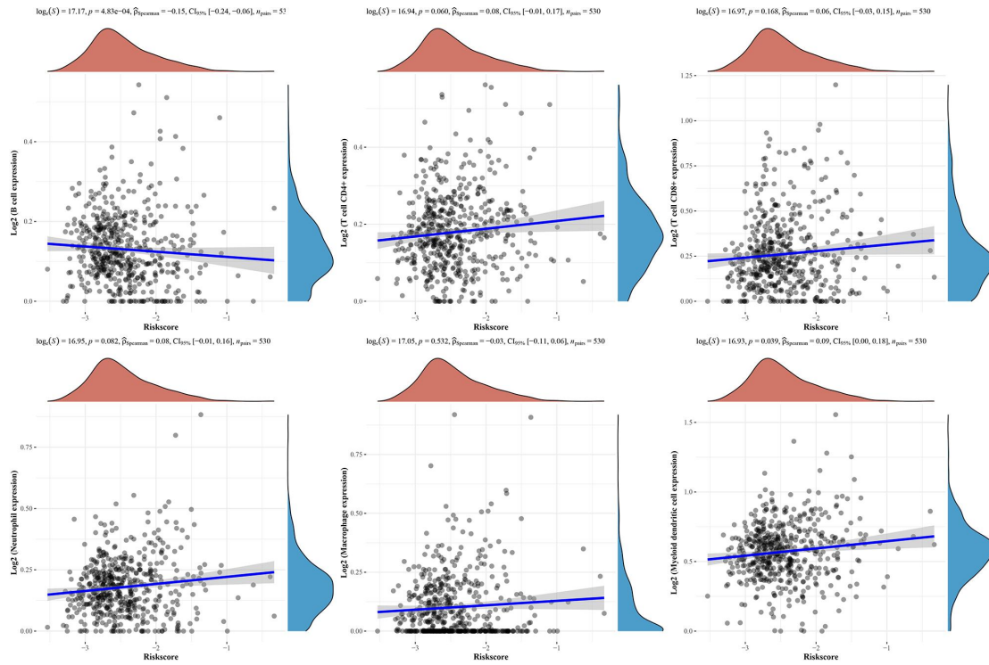
Fig.S4.3 The correlation of CRG_score with immune cells was analyzed using TIMER
