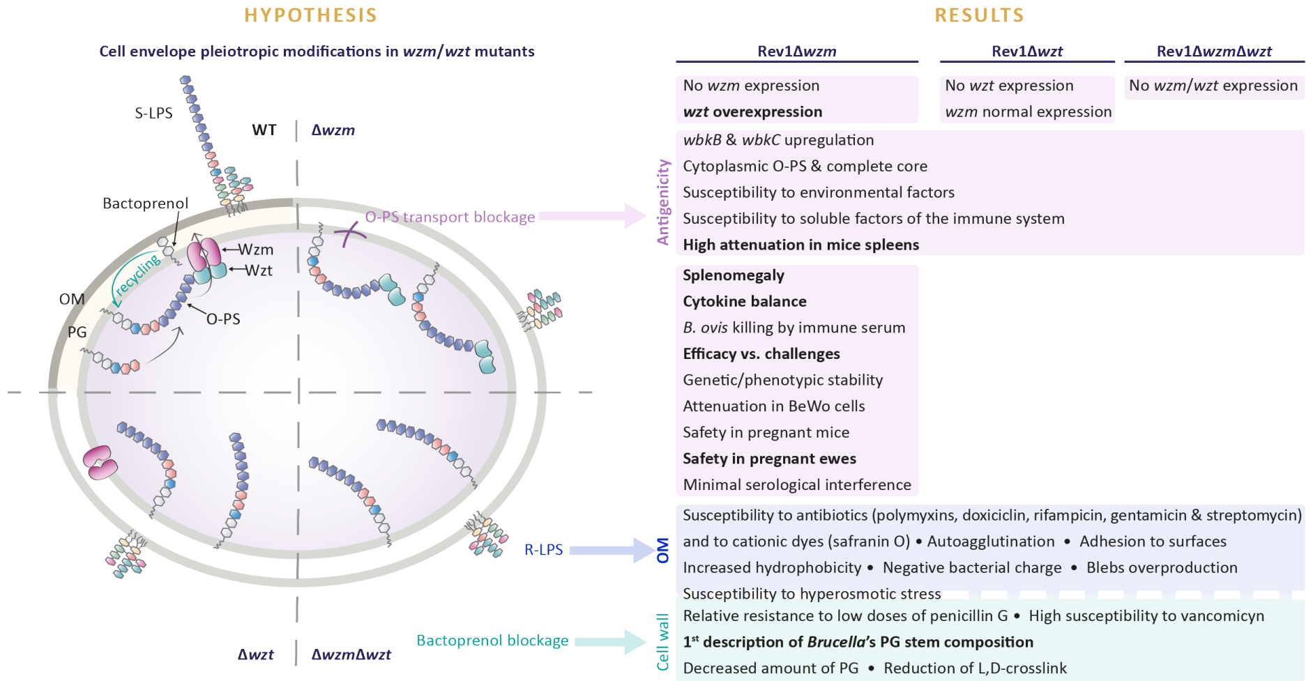
Supplementary Figure 2. Schematic representation of the starting hypothesis (left) and the main results obtained (right) concerning bacterial envelope changes associated with antigenicity, OM and cell wall in Rev1 wzm/wzt mutants.
