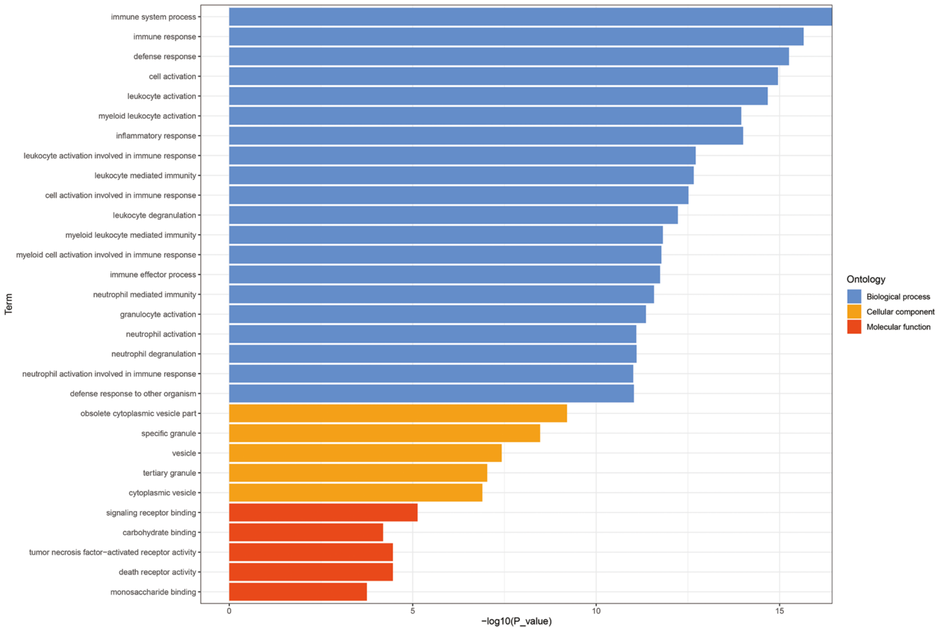
GO enrichment analysis of up-regulated DEGs between geriatric and adults.
