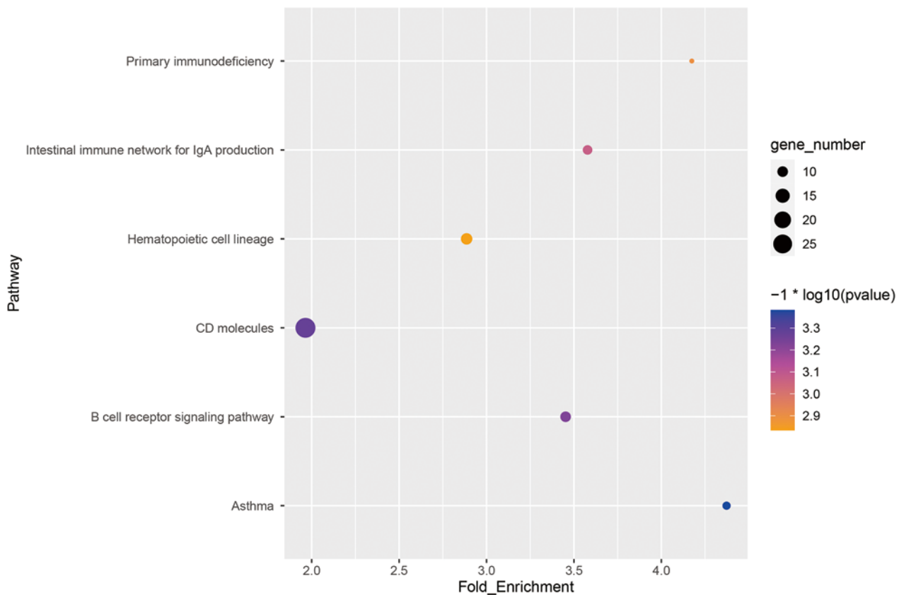
KEGG enrichment analysis of down-regulated DEGs between geriatric and adults.
