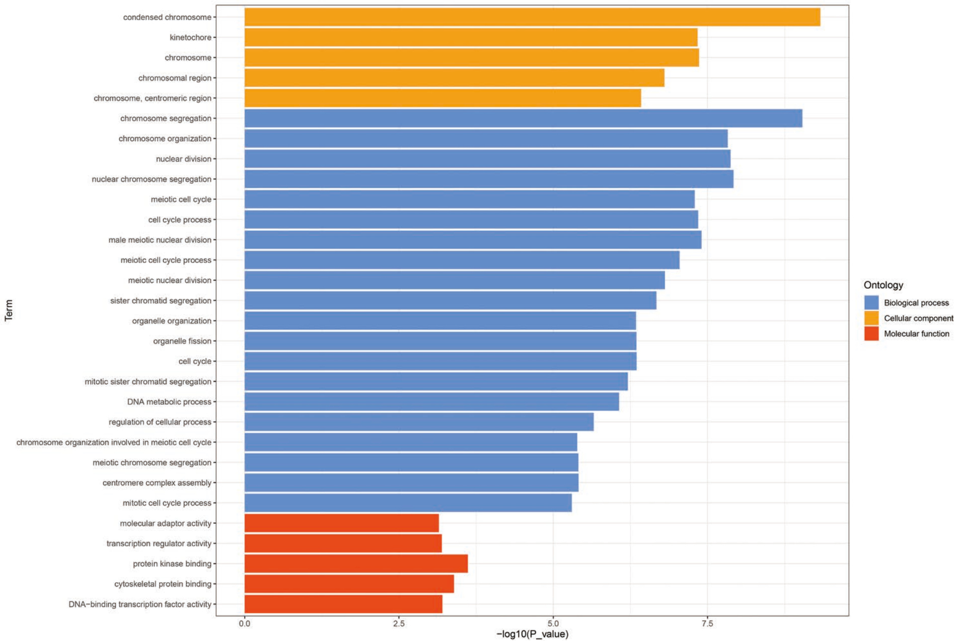
GO enrichment analysis of down-regulated DEGs between geriatric and adults.
