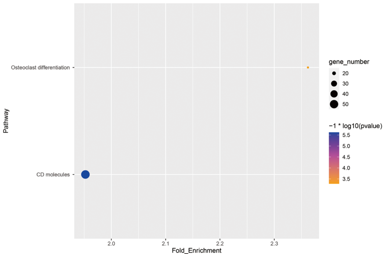
KEGG enrichment analysis of up-regulated DEGs between geriatric and adults.
