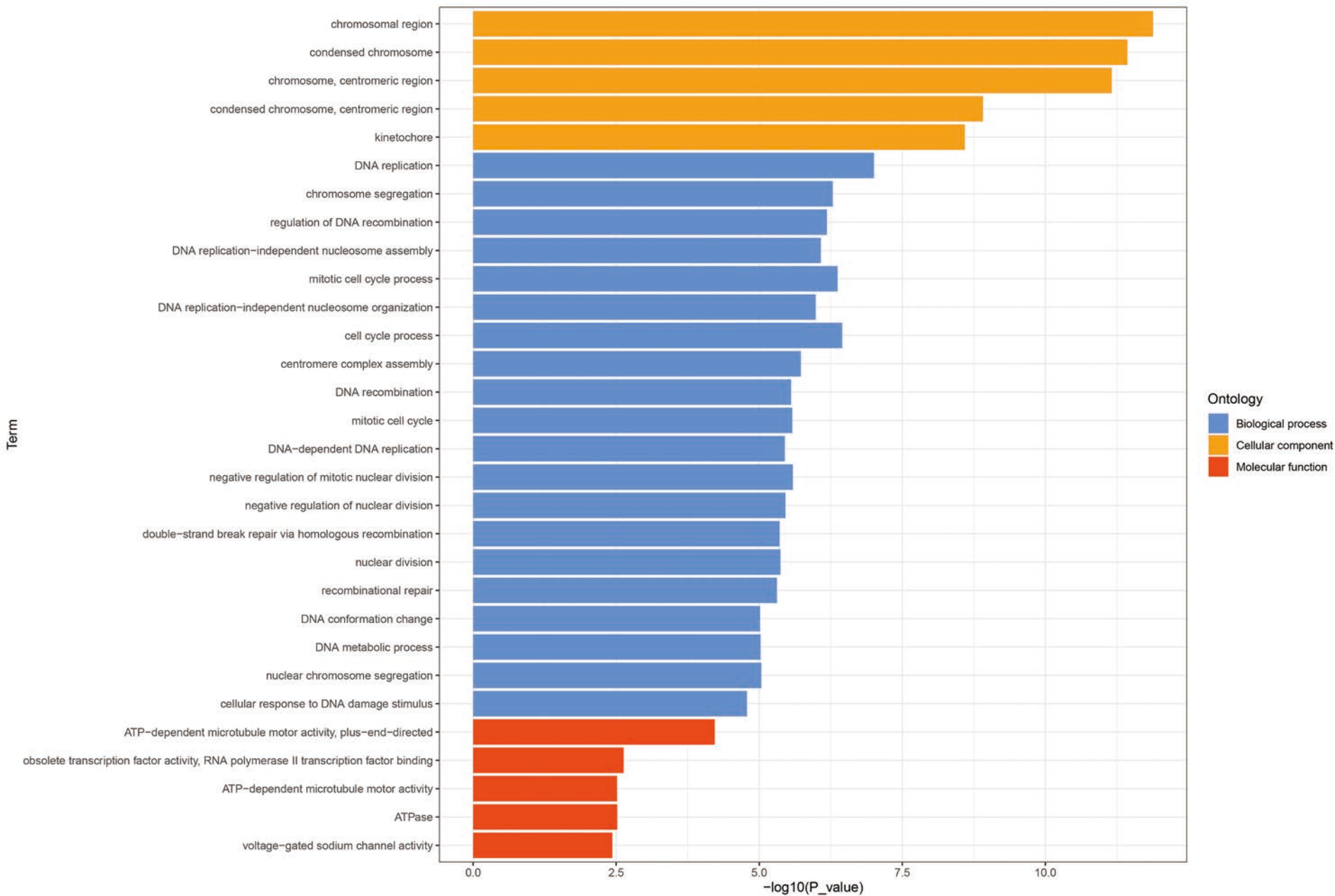
GO enrichment analysis of up-regulated DEGs between adults and juveniles.
