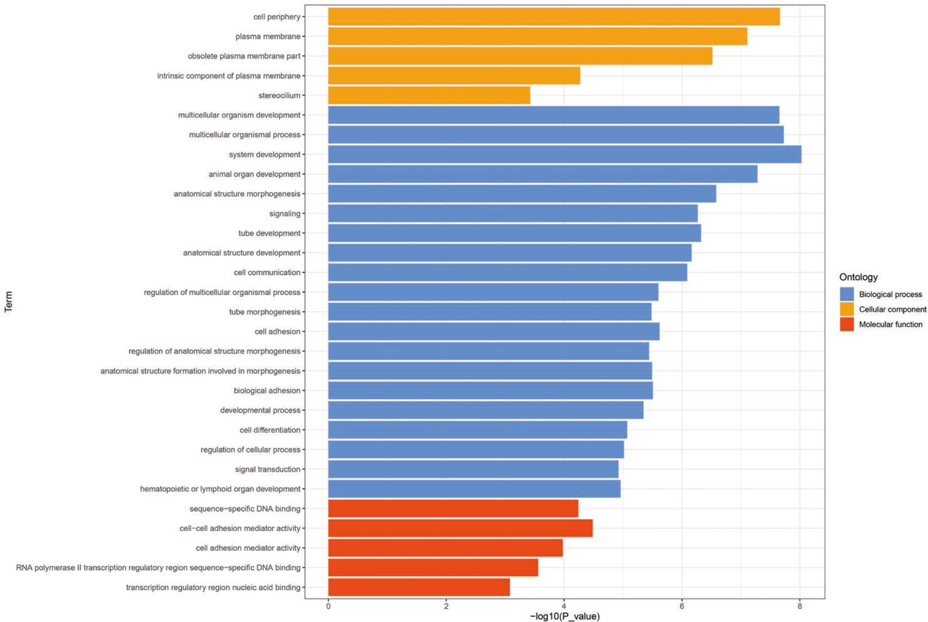
GO enrichment analysis of down-regulated DEGs between adults and juveniles.
