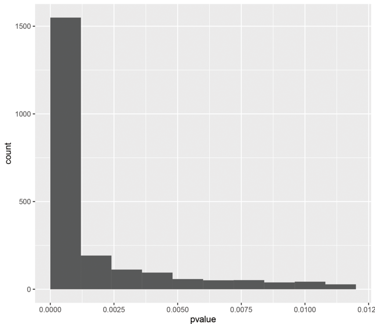
P-values frequency distribution of DEGs between geriatric and adults.
