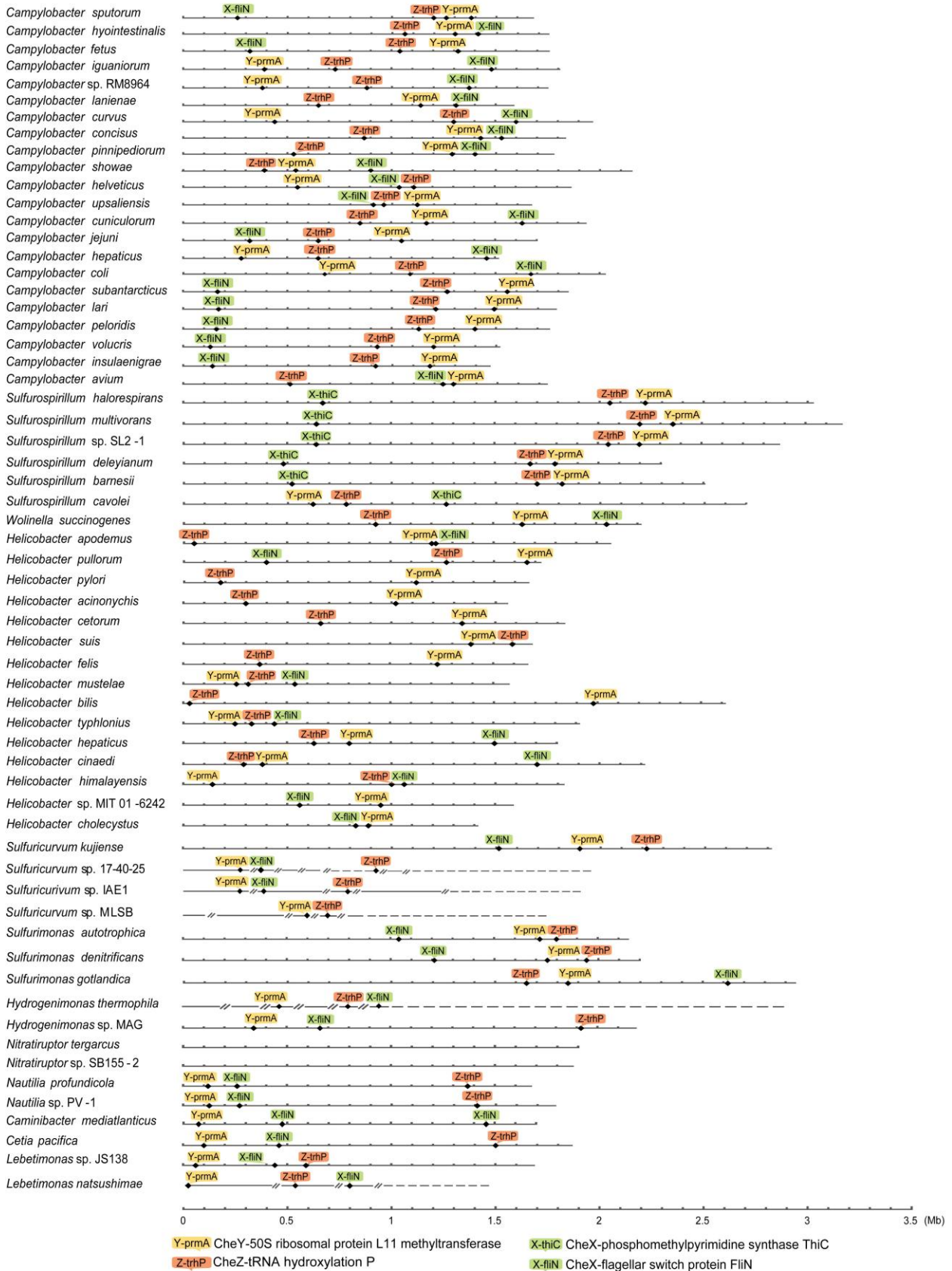
S1 Fig. The conserved gene order of F3 chemosensory class genes cheX , cheY , and cheZ . Abbreviations: X- fliN , CheX-flagellar switch protein FliN; Y- prmA , CheY-50S ribosomal protein L11 methyltransferase; Z- trhP , CheZ-tRNA hydroxylation P.
