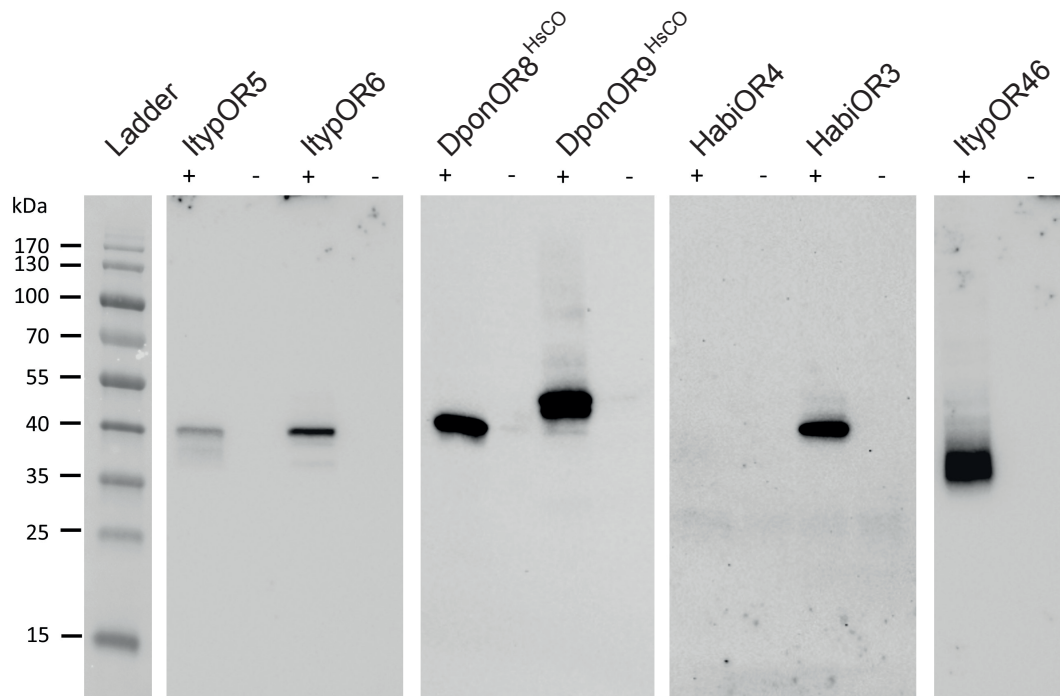
Supplementary Figure 1. Results from Western blot analyses of V5-tagged odorant receptors (ORs) from TREx/HEK293 cells. Included are ORs from Ips typographus (ItypOR5 and ItypOR6), Dendroctonus ponderosae (DponOR8 and DponOR9, expressed from Homo sapiens codon-optimized, 'HsCO', genes), and Hylobius abietis (HabiOR3 and HabiOR4). Proteins were only detected from cells induced (+) to express the OR genes, and not from non-induced (-) control cells, indicating proper regulation by the repression system. ItypOR46 was included as a positive control (see Yuvaraj et al., 2021).
