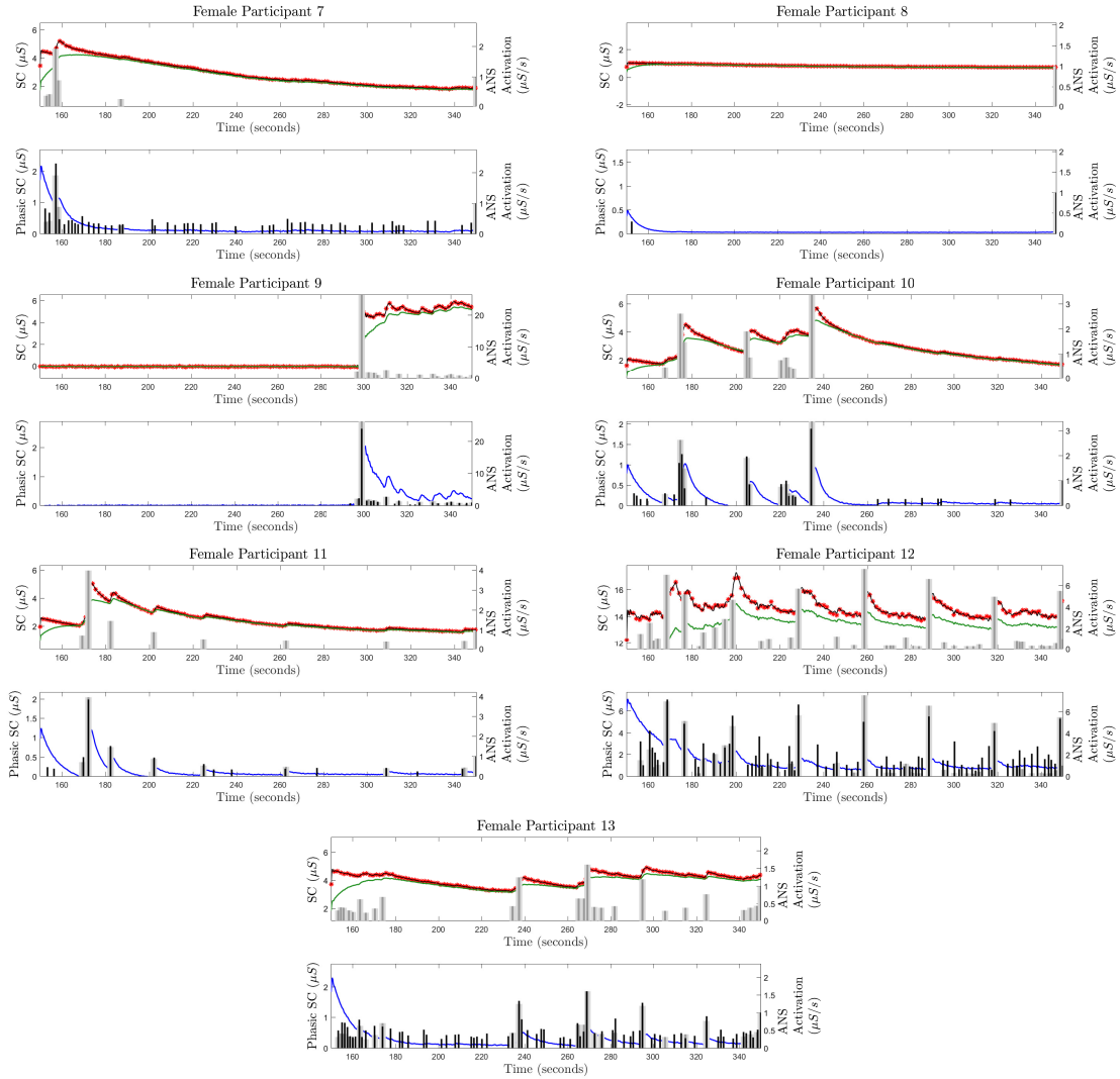
Fig S6. Deconvolution Results From the Simulated SC Signals with 25 dB SNR for Female Participant 7 to 13: In each of the panels, i) the top sub-panel shows the ground truth for SC signal (red stars), the reconstructed SC signal (black solid curve), the estimated tonic component (green solid curve), and ground truth for the ANS activation (gray vertical lines); ii) the bottom sub-panel shows the estimated phasic component (blue solid curve), estimated ANS activation timings and amplitudes (black vertical lines) and the ground truth ANS activation (gray vertical lines).
