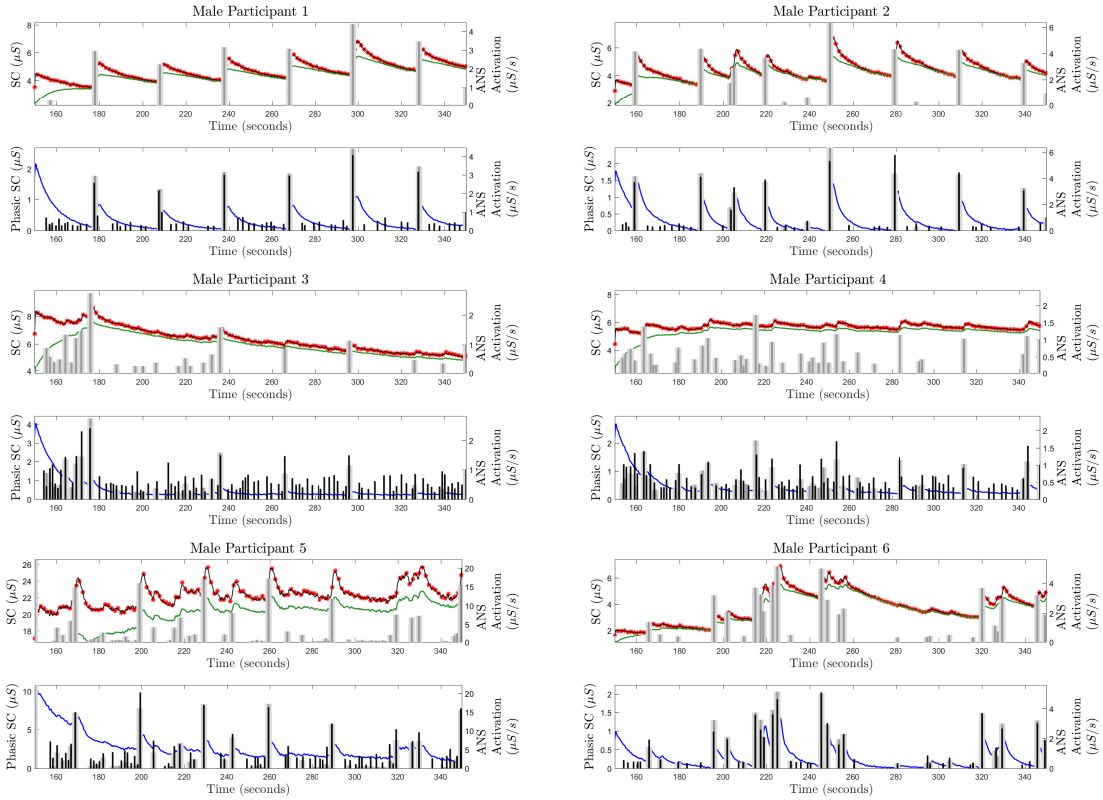
Fig S7. Deconvolution Results From the Simulated SC Signals with 25 dB SNR for Male Participant 1 to 6: In each of the panels, i) the top sub-panel shows the ground truth for SC signal (red stars), the reconstructed SC signal (black solid curve), the estimated tonic component (green solid curve), and ground truth for the ANS activation (gray vertical lines); ii) the bottom sub-panel shows the estimated phasic component (blue solid curve), estimated ANS activation timings and amplitudes (black vertical lines) and the ground truth ANS activation (gray vertical lines).
