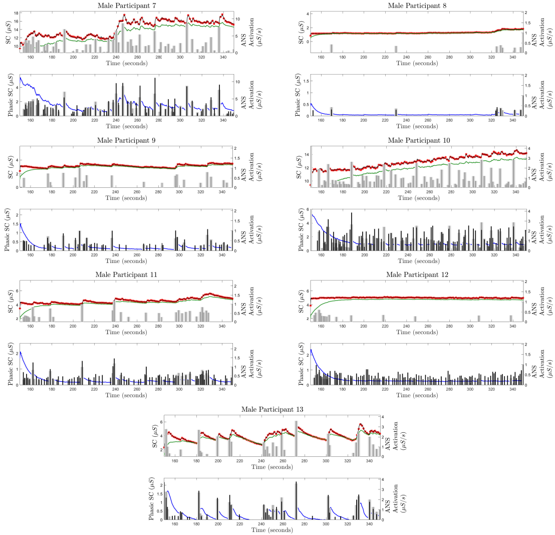
Fig S8. Deconvolution Results From the Simulated SC Signals with 25 dB SNR for Male Participant 7 to 13: In each of the panels, i) the top sub-panel shows the ground truth for SC signal (red stars), the reconstructed SC signal (black solid curve), the estimated tonic component (green solid curve), and ground truth for the ANS activation (gray vertical lines); ii) the bottom sub-panel shows the estimated phasic component (blue solid curve), estimated ANS activation timings and amplitudes (black vertical lines) and the ground truth ANS activation (gray vertical lines).
