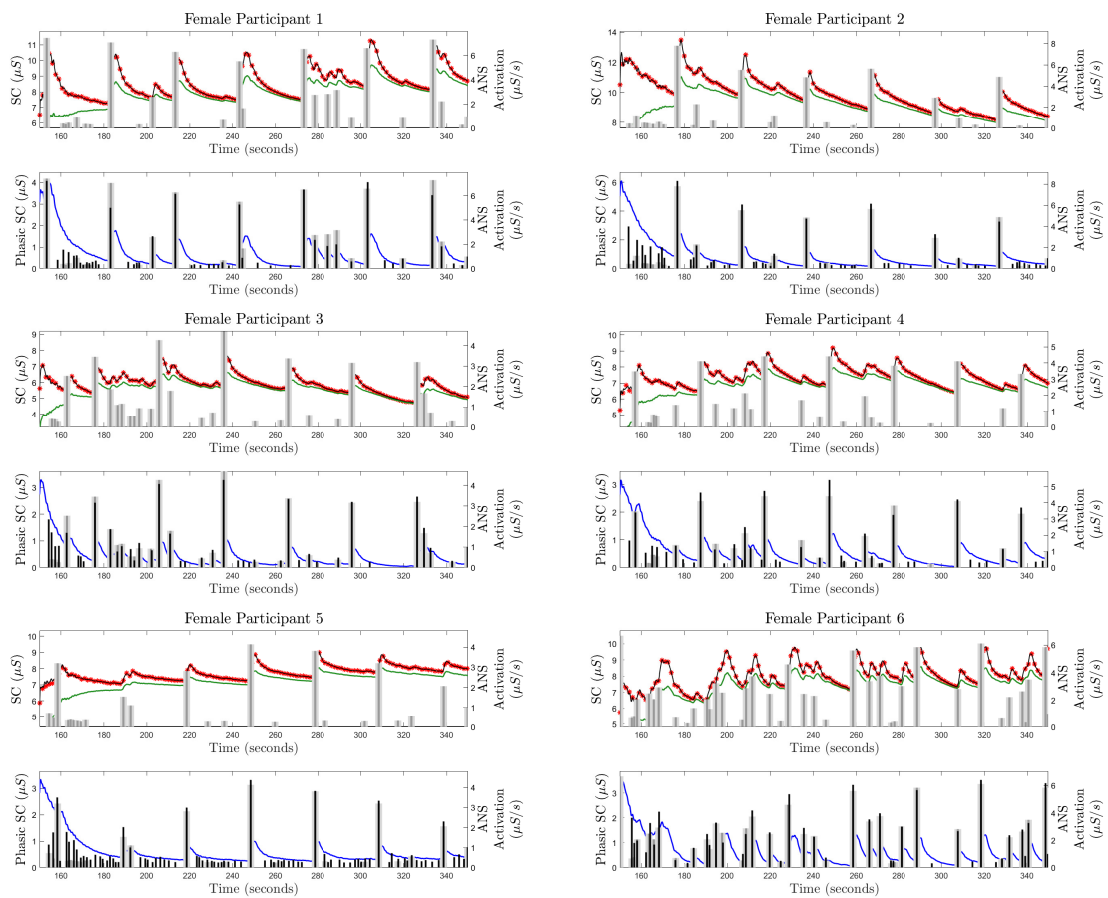
Fig S13. Deconvolution Results From the Simulated SC Signals with 25 dB SNR with Pink Noise for Female Participant 1 to 6: In each of the panels, i) the top sub-panel shows the ground truth for SC signal (red stars), the reconstructed SC signal (black solid curve), the estimated tonic component (green solid curve), and ground truth for the ANS activation (gray vertical lines); ii) the bottom sub-panel shows the estimated phasic component (blue solid curve), estimated ANS activation timings and amplitudes (black vertical lines) and the ground truth ANS activation (gray vertical lines).
