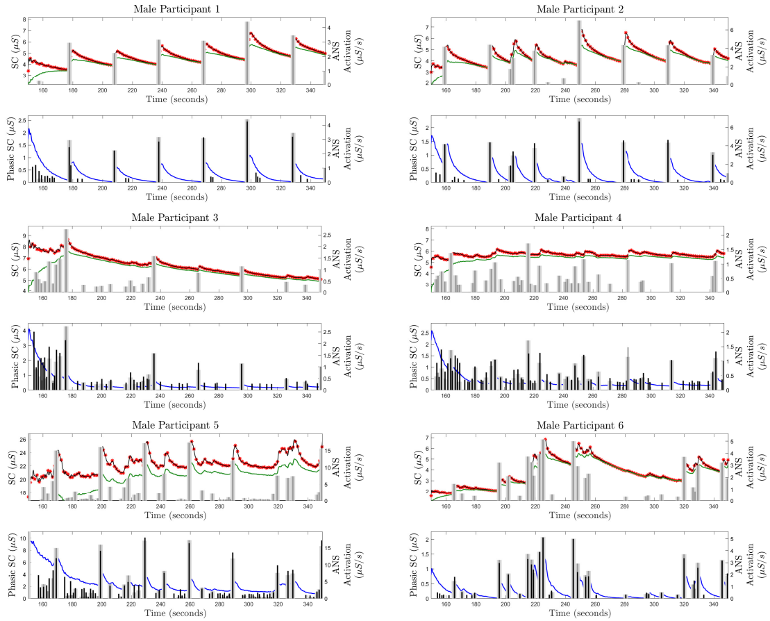
Fig S15. Deconvolution Results From the Simulated SC Signals with 25 dB SNR with Pink Noise for Male Participant 1 to 6: In each of the panels, i) the top sub-panel shows the ground truth for SC signal (red stars), the reconstructed SC signal (black solid curve), the estimated tonic component (green solid curve), and ground truth for the ANS activation (gray vertical lines); ii) the bottom sub-panel shows the estimated phasic component (blue solid curve), estimated ANS activation timings and amplitudes (black vertical lines) and the ground truth ANS activation (gray vertical lines).
