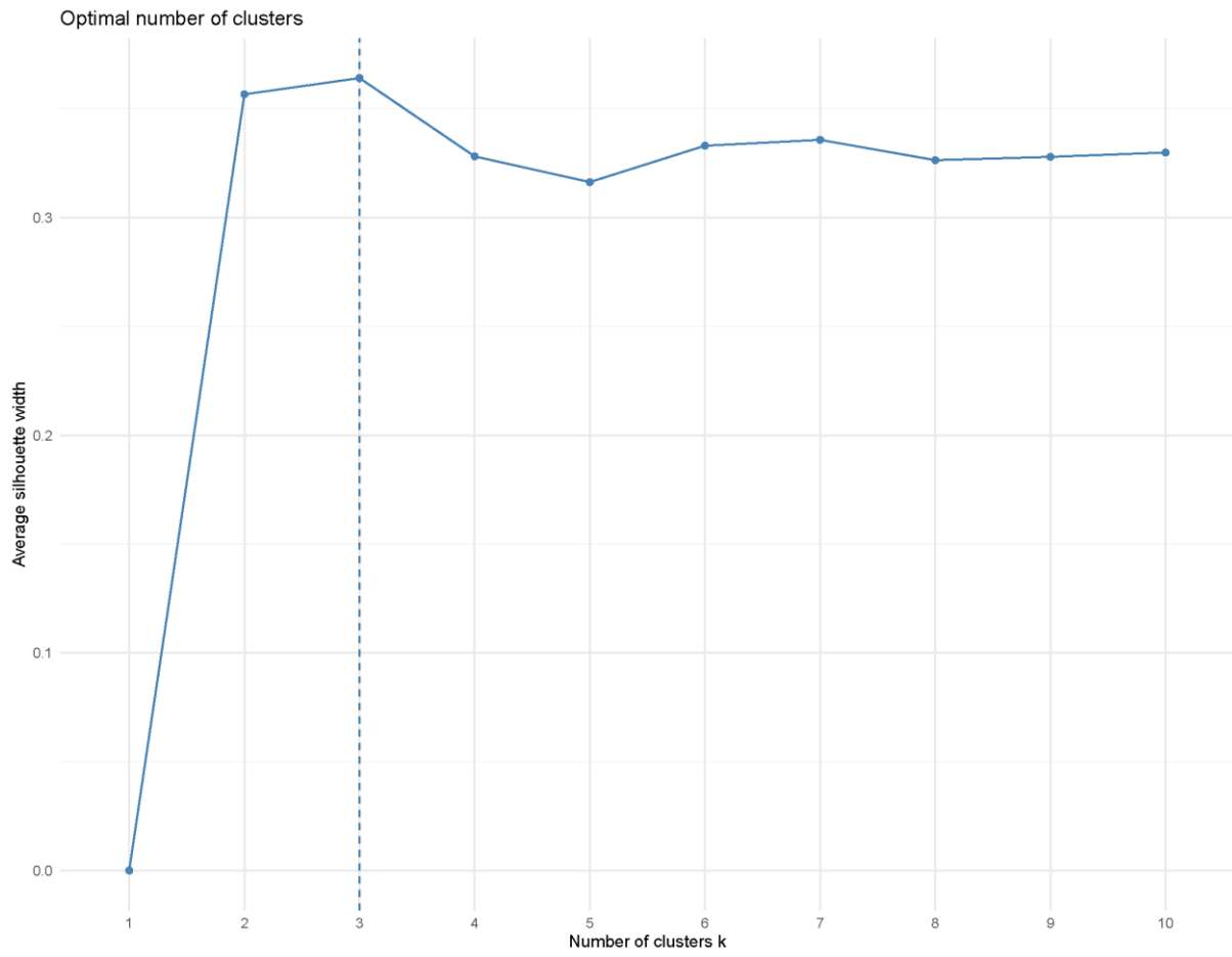
Fig. S1 Silhouette width by number of clusters
