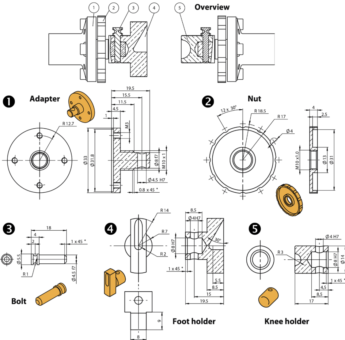
Supplementary Figure 1: Example of loading device with dimensions for the foot and knee fixtures 42 .
