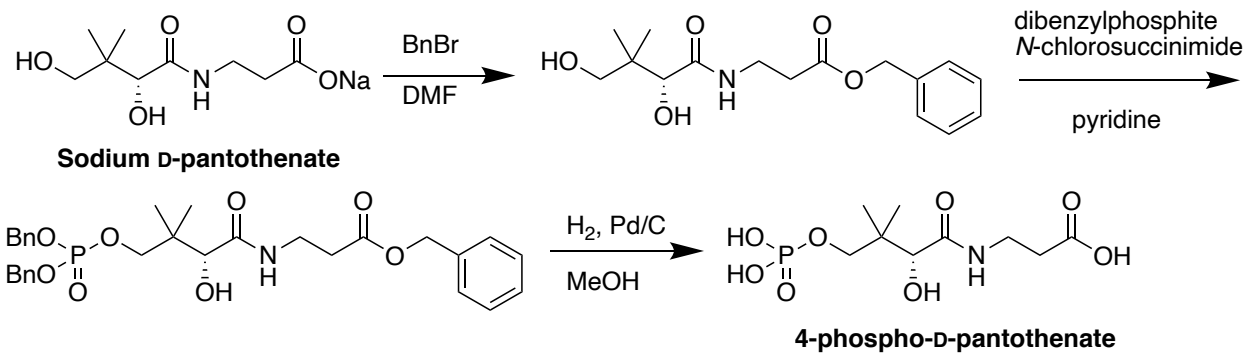
Supplemental Information Fig. 2. Diagram of steps for 4 1 -phosphopantothenate synthesis.
