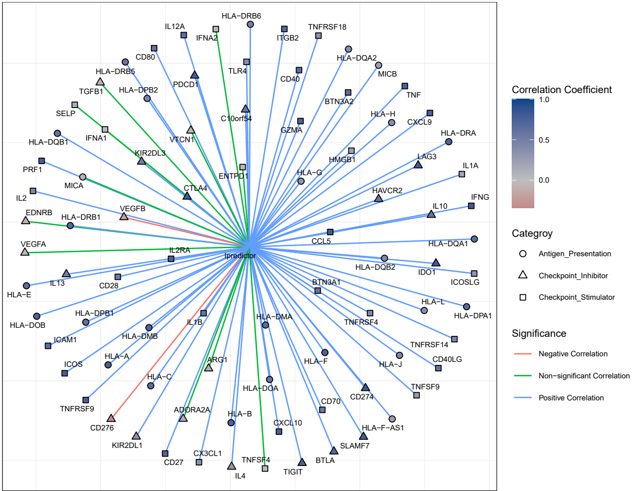
Supplementary Figure 11. Association between the PS and expression of antigen presentation genes and immune checkpoint genes.
