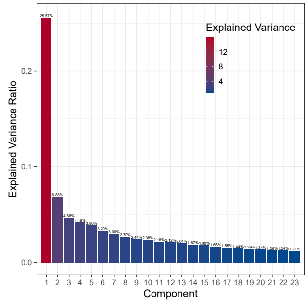
Supplementary Figure 3. Feature engineering. (A) Feature selection using Spearman rank correlation test. (B) Dimensionality reduction via PCA.
