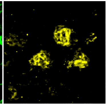
Alexa 647
