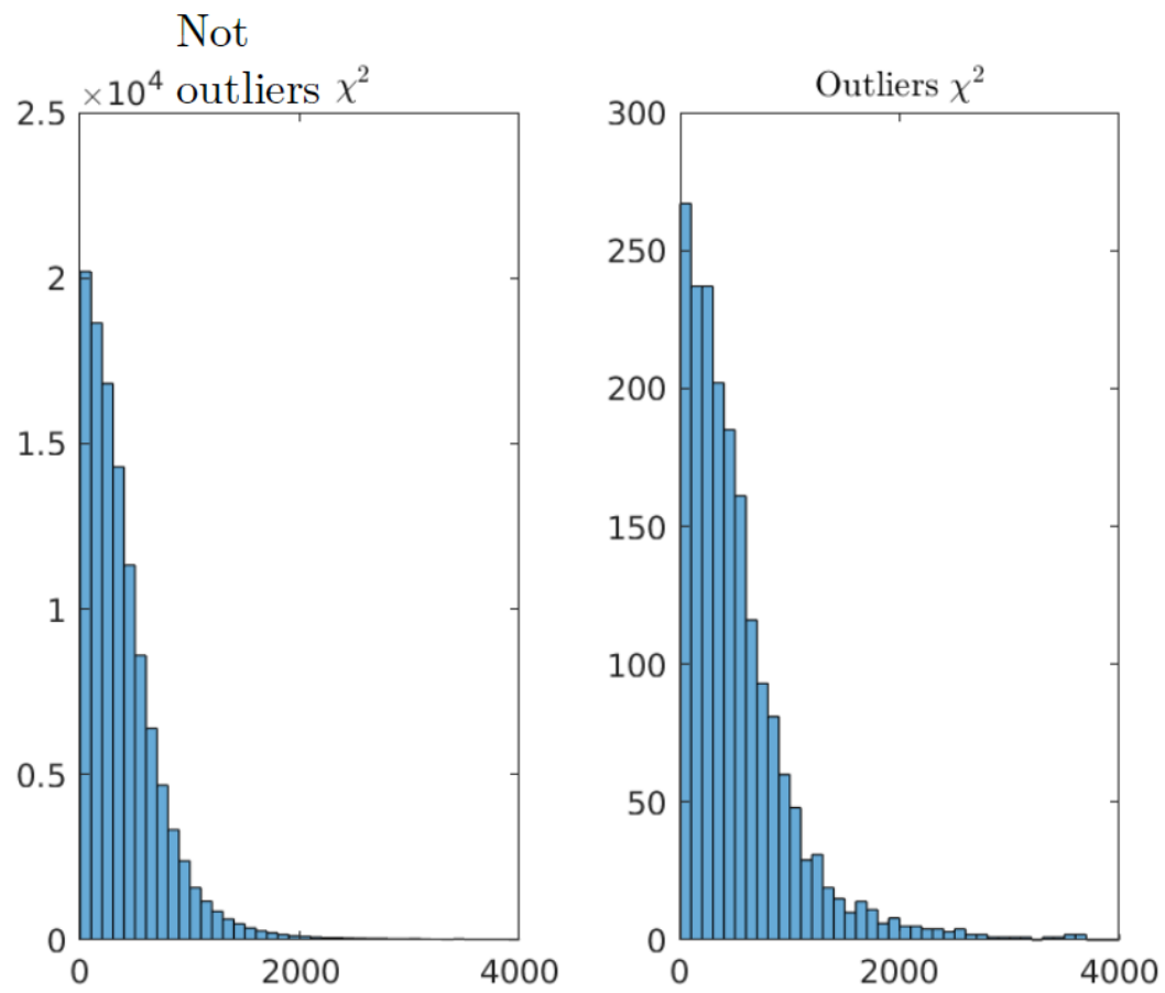
Figure 1: : Examples of histograms of quality of fit of the outliers excluded from the LME fit (on the right), and the rest of the voxels (on the left).
