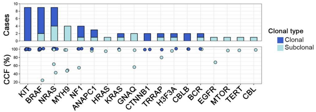
Fig. S14. Graphical representation of distribution of the CCF for acral melanoma driver SNVs.
