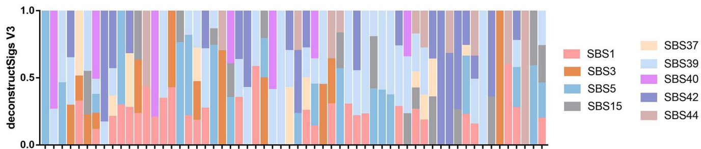
Fig. S6. The relative contribution of mutation signatures analyzed by deconstructSigs. The results were assigned to COSMIC V3.2. Signatures were differentiated by colors.
