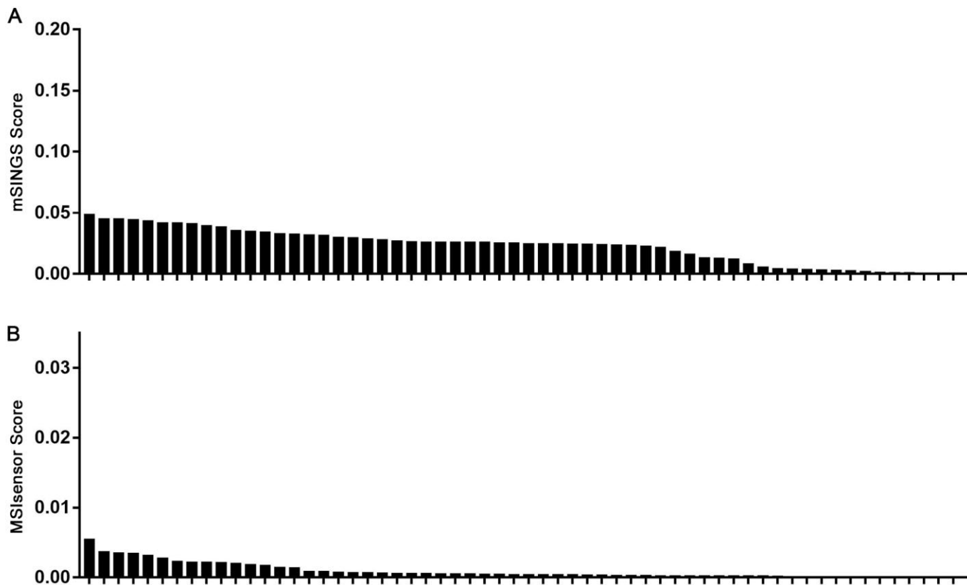
Fig. S7. Fraction of unstable microsatellite loci identified by NGS predicts MSI status. (A) The MSI assessed by mSINGS. And the cutoff of mSINGS score was 0.2. (B) The MSI assessed by MSIsensor. And the cutoff of MSIsensor score was 0.035.
