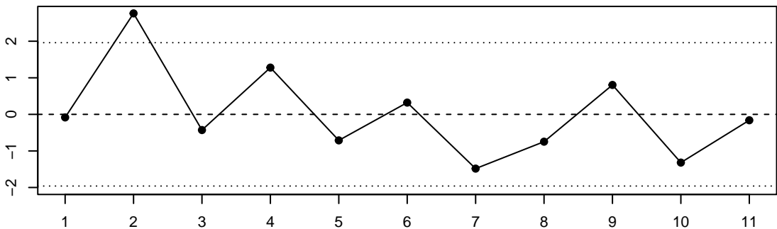
rstudent
