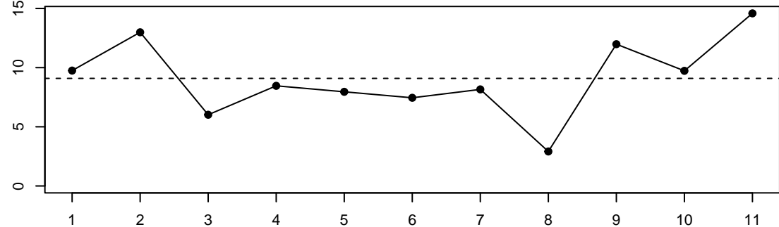
weight
