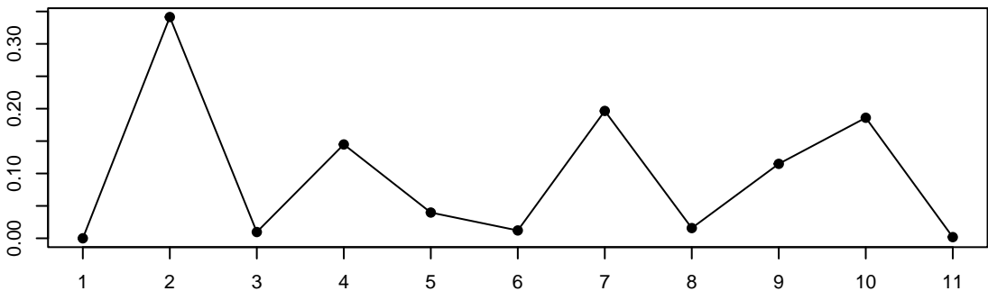
cook.d
