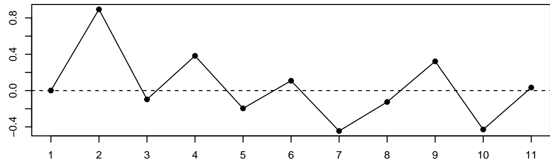
dffits
