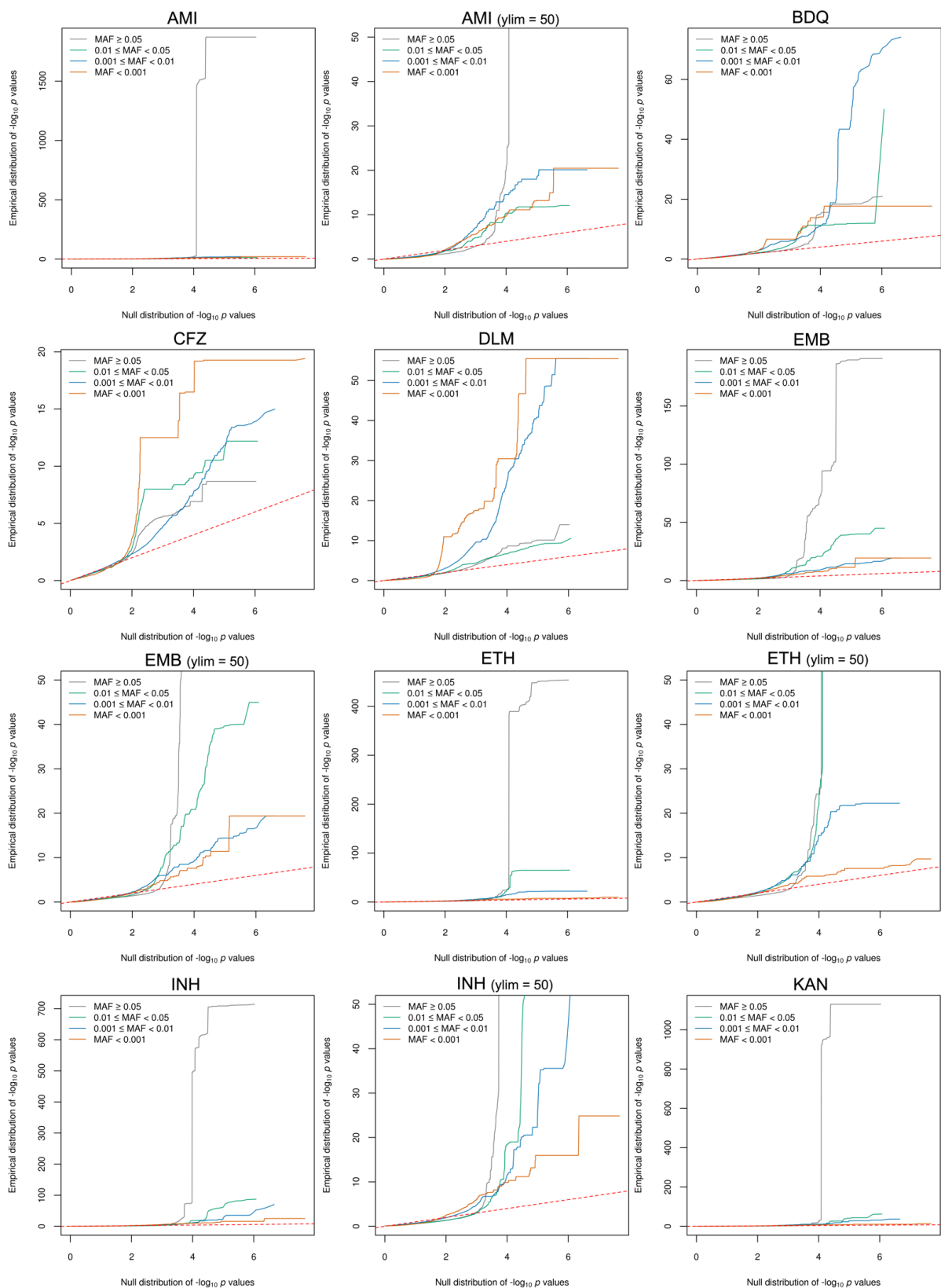
S3 Fig. QQ plots for the oligopeptide analyses, part A. Comparing the empirical distribution of p-values to the
