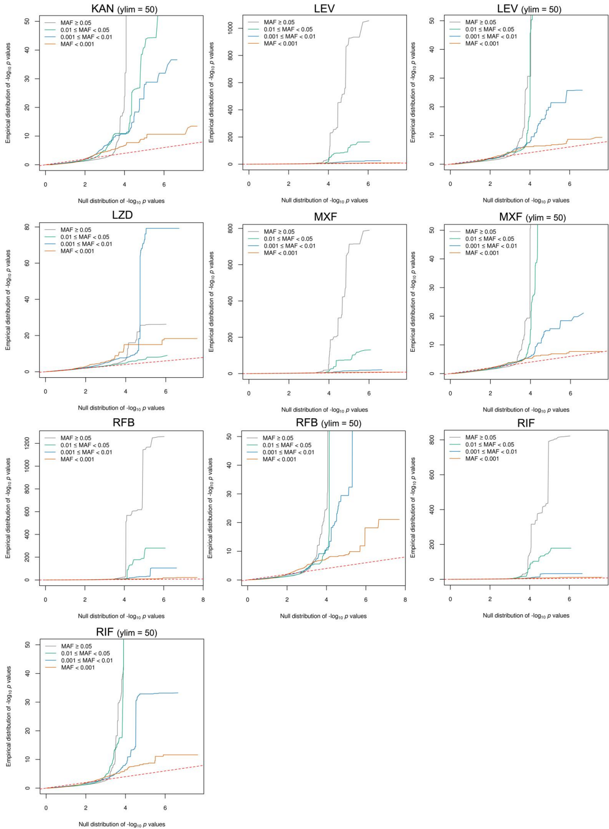
S4 Fig. QQ plots for the oligopeptide analyses, part B. Comparing the empirical distribution of p-values to the
