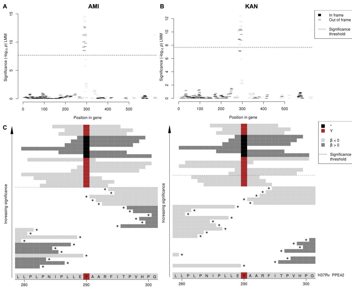
S9 Fig. Variants in PPE42 associated with amikacin (AMI) and kanamycin (KAN) MIC. Manhattan plots showing the oligopeptide association results for the PPE42 coding region A amikacin and B kanamycin, and oligopeptide alignment plots showing close ups of the significant region in PPE42 for C amikacin and D kanamycin. Black dashed lines indicate the Bonferroni-corrected significance thresholds. In the Manhattan plots, oligopeptides are coloured by the reading frame that they align to, black for the correct reading frame for PPE42 . Oligopeptides assigned to the region but did not align using BLAST are shown in grey on the right hand side of the plots. In the oligopeptide alignment plots, the H37Rv reference codons are shown at the bottom of the figure, grey for an invariant site, coloured at variant site positions. The oligopeptides that aligned to the region are plotted from least significant at the bottom to most significant at the top. The background colour of the oligopeptides represents the direction of the b estimate, light grey when b < 0 (associated with lower MIC), dark grey when b > 0 (associated with higher MIC). Oligopeptides are coloured by their amino acid residue at all variant positions. Oligopeptides below the MAF threshold and not included in the analysis, but visualised here for signal interpretation, are marked by *s.
