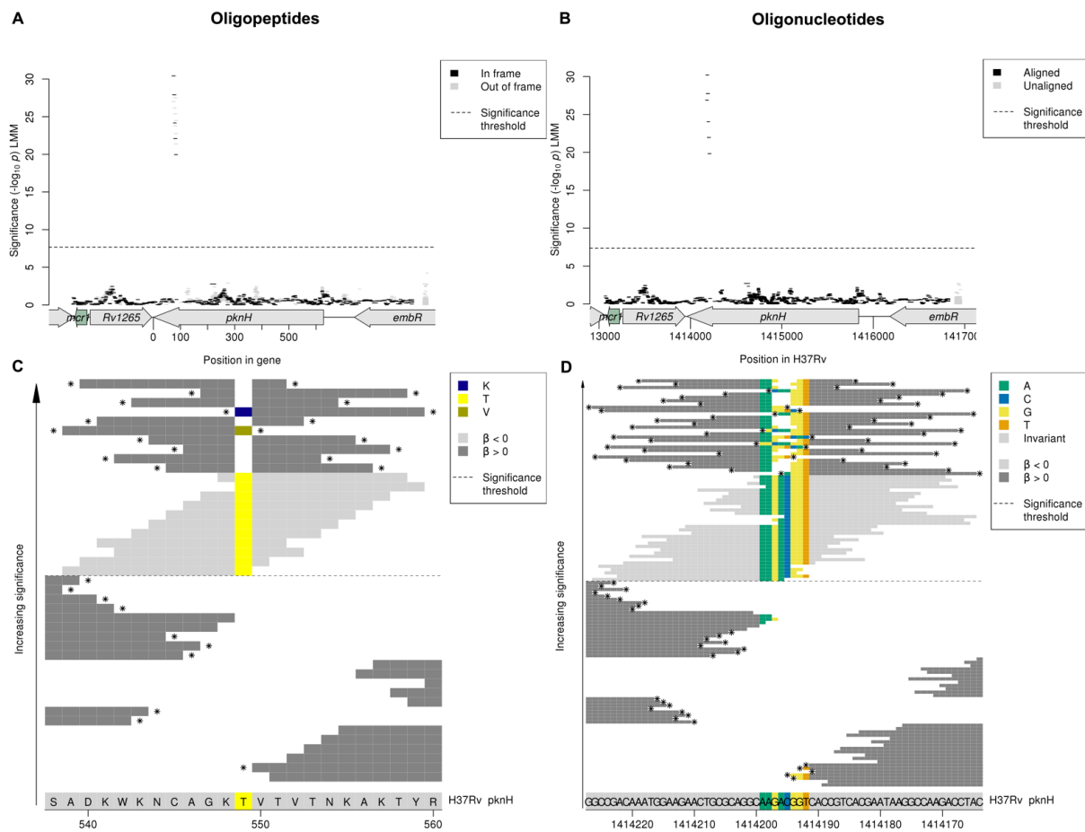
S15 Fig. Variants in pknH associated with delamanid MIC. Manhattan plots showing the association results for the pknH coding region for the A oligopeptides and B oligonucleotides, and alignment plots showing close ups of the significant region in pknH for the C oligopeptides D oligonucleotides. The black dashed lines indicate the Bonferroni-corrected significance thresholds. In the Manhattan plots, oligopeptides are coloured by the reading frame that they align to, black for the correct reading frame for pknH . Oligo-peptides and nucleotides assigned to the region but did not align using BLAST are shown in grey on the right hand side of the plots. In the alignment plots, the H37Rv reference alleles are shown at the bottom of the figure, grey for an invariant site, coloured at variant site positions. The oligo-peptides and nucleotides that aligned to the region are plotted from least significant at the bottom to most significant at the top. The background colour of the oligo-peptides and nucleotides represents the direction of the b estimate, light grey when b < 0 (associated with lower MIC), dark grey when b > 0 (associated with higher MIC). Oligo-peptides and nucleotides are coloured by their allele at all variant positions. Oligo-peptides and nucleotides below the MAF threshold and not included in the analysis, but visualised here for signal interpretation, are marked by *s.
