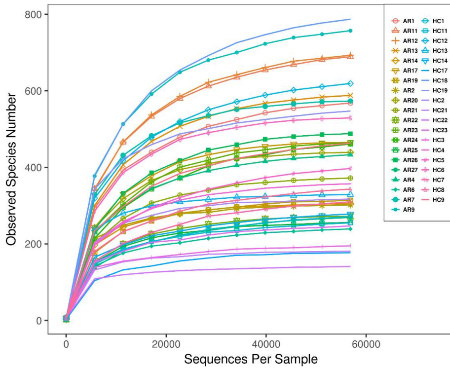
Figure S1: Species diversity curve -- dilution curve.
