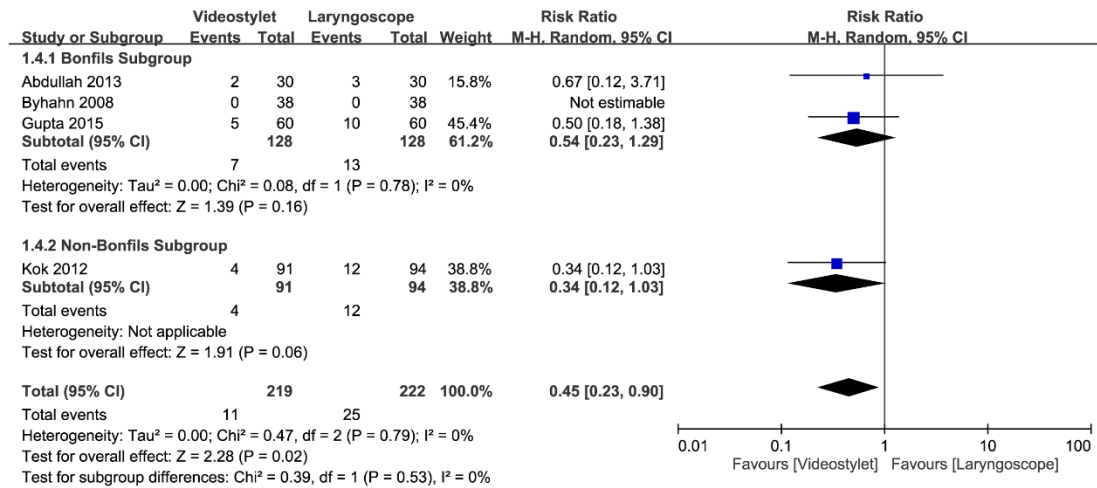
Supplementary Figure 3. Forest plot comparing the risk of sore throat between video-stylet and laryngoscope groups. CI, confidence interval; RR, risk ratio; M-H, Mantel–Haenszel.
