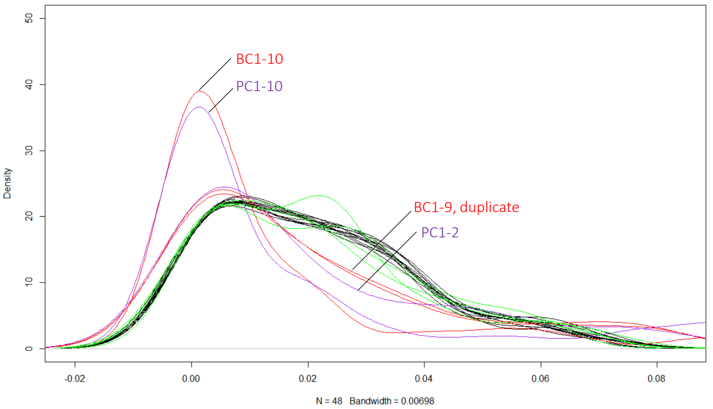
Densityplot of sequence-read distribution mFAST-SeqS on single cell WGA
