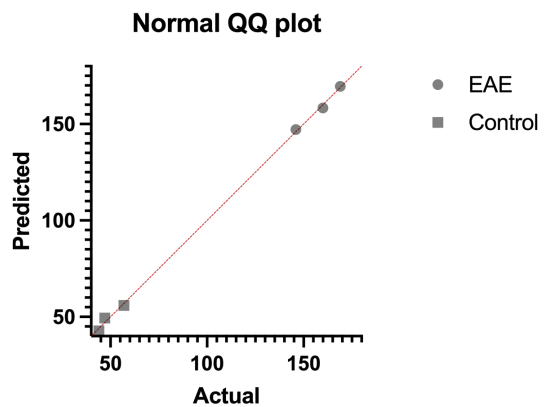
E2.8. Q-Q plot
