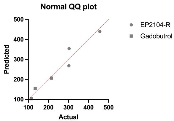
E2.9. Q-Q plot
