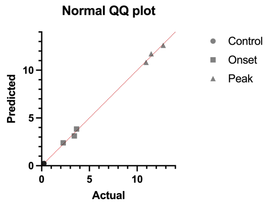
E2.6. Q-Q plot
