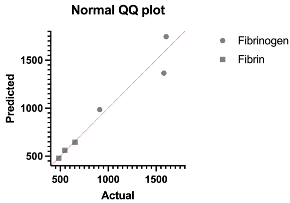
E2.1. Q-Q plot
