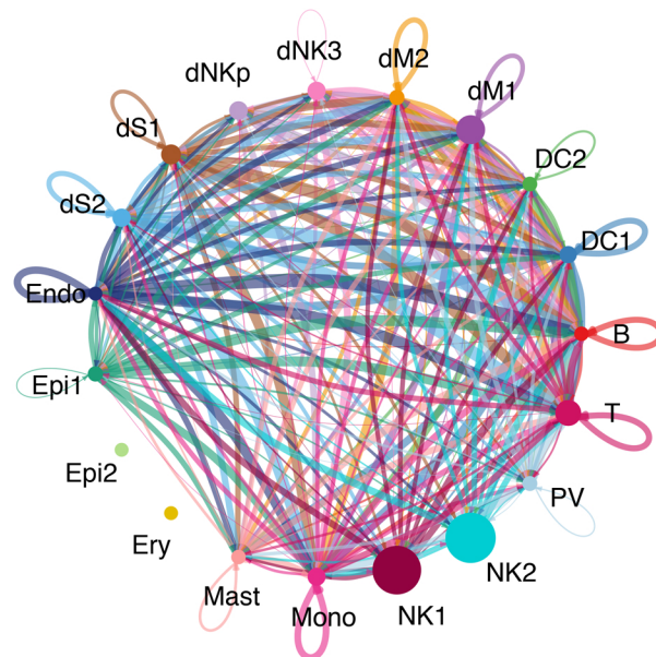
Interaction weights/strength
