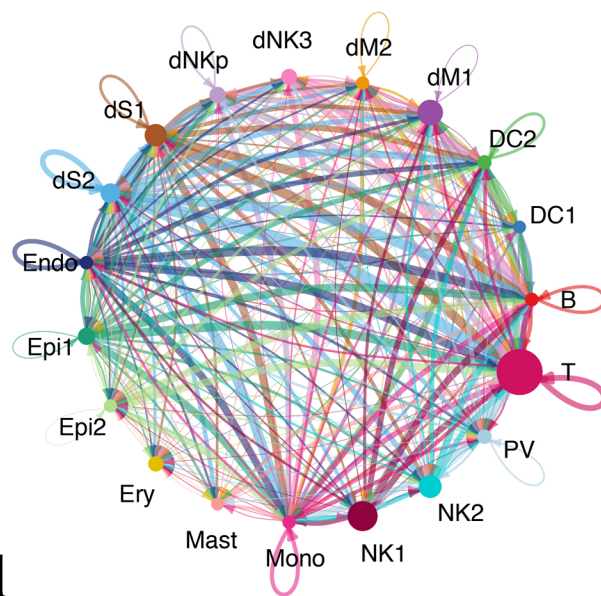
Interaction weights/strength
