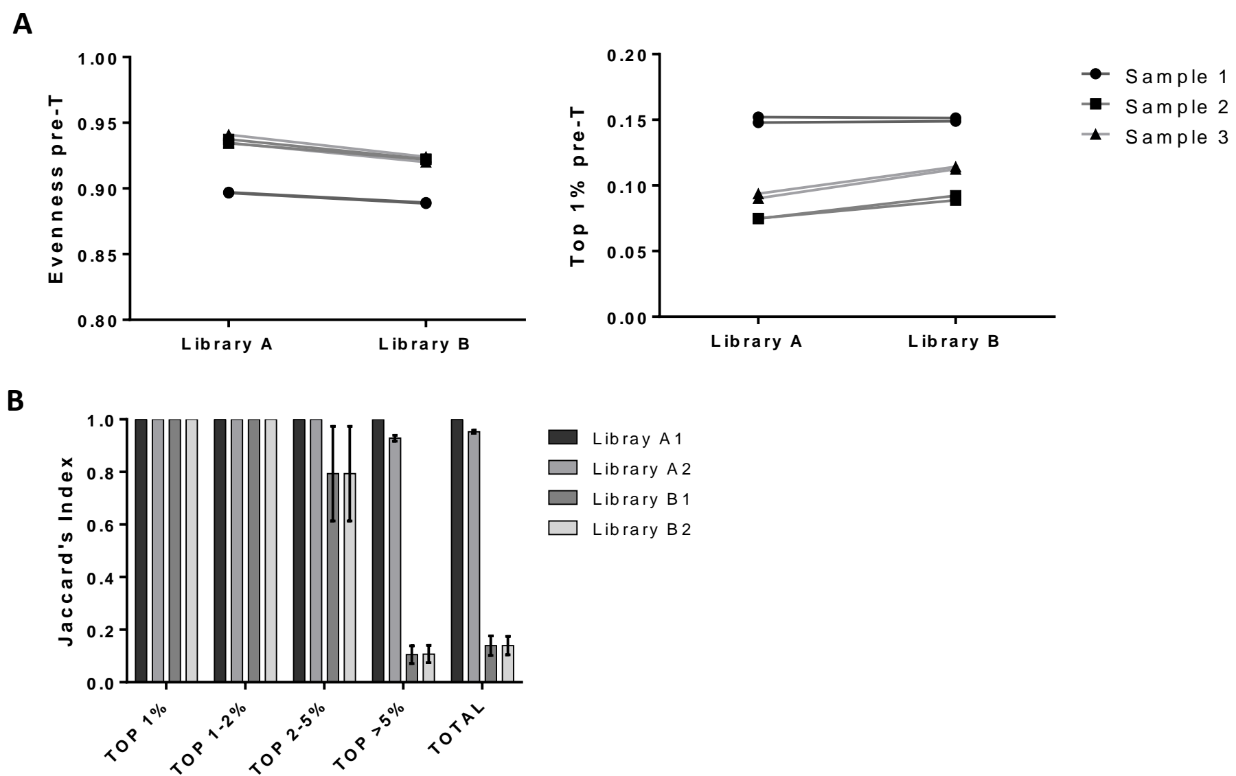
Supplementary Figure S3. A. Stability of evenness and top 1% across technical replicates. B. Clonal reproducibility in frequency ranks between sequencing replicates or libraries.
